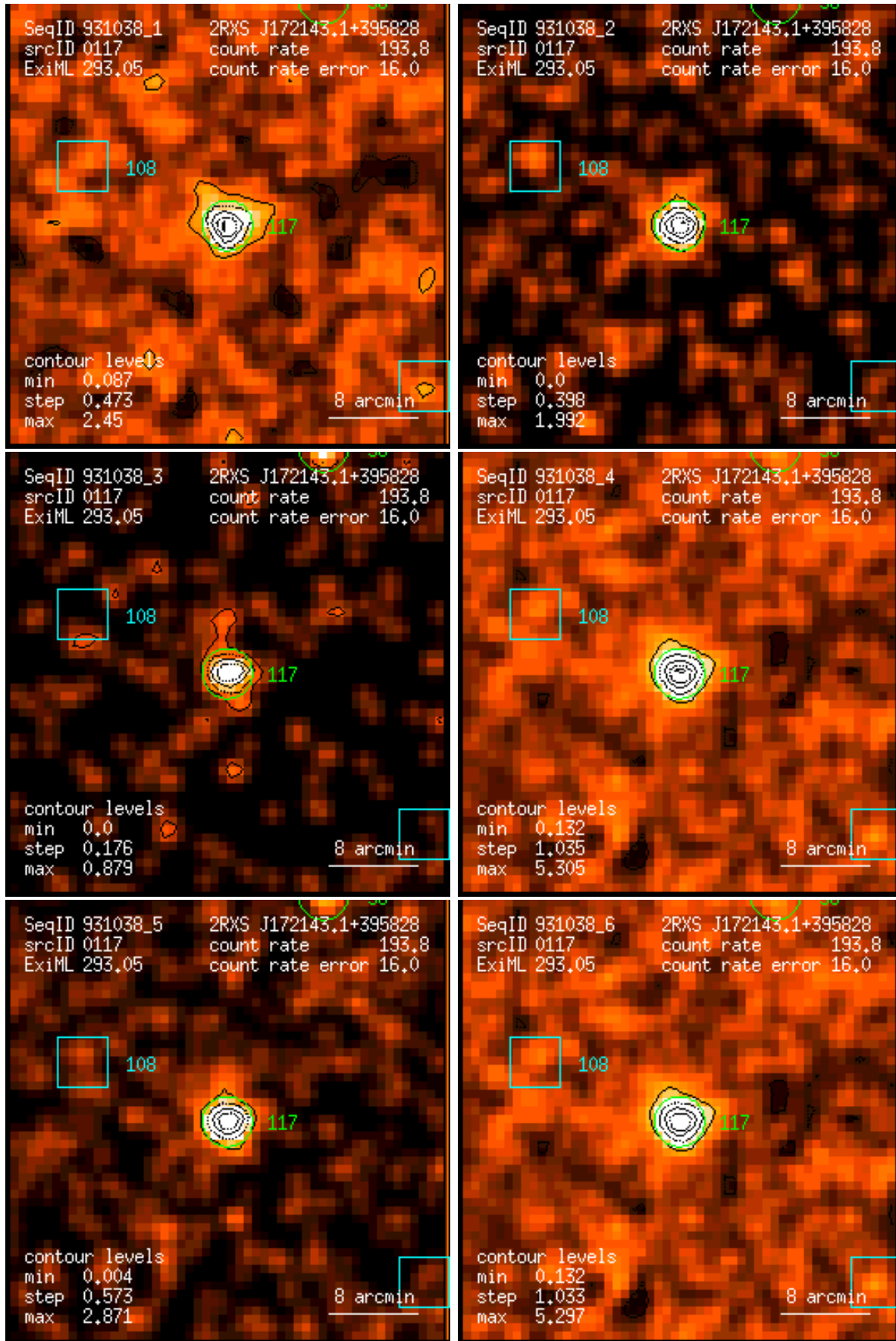
Figure 117: RASS 931038: detection 0117: band rate images, Gaussian filter: (1) PSPC channels 11 – 41, (2) 52 – 90, (3) 91 – 201, (4) 11 – 235, (5) 52 – 201, (6) 11 – 201. Broad band rates in counts/ks. Band rate contour levels in counts/ks/arcmin 2 .
