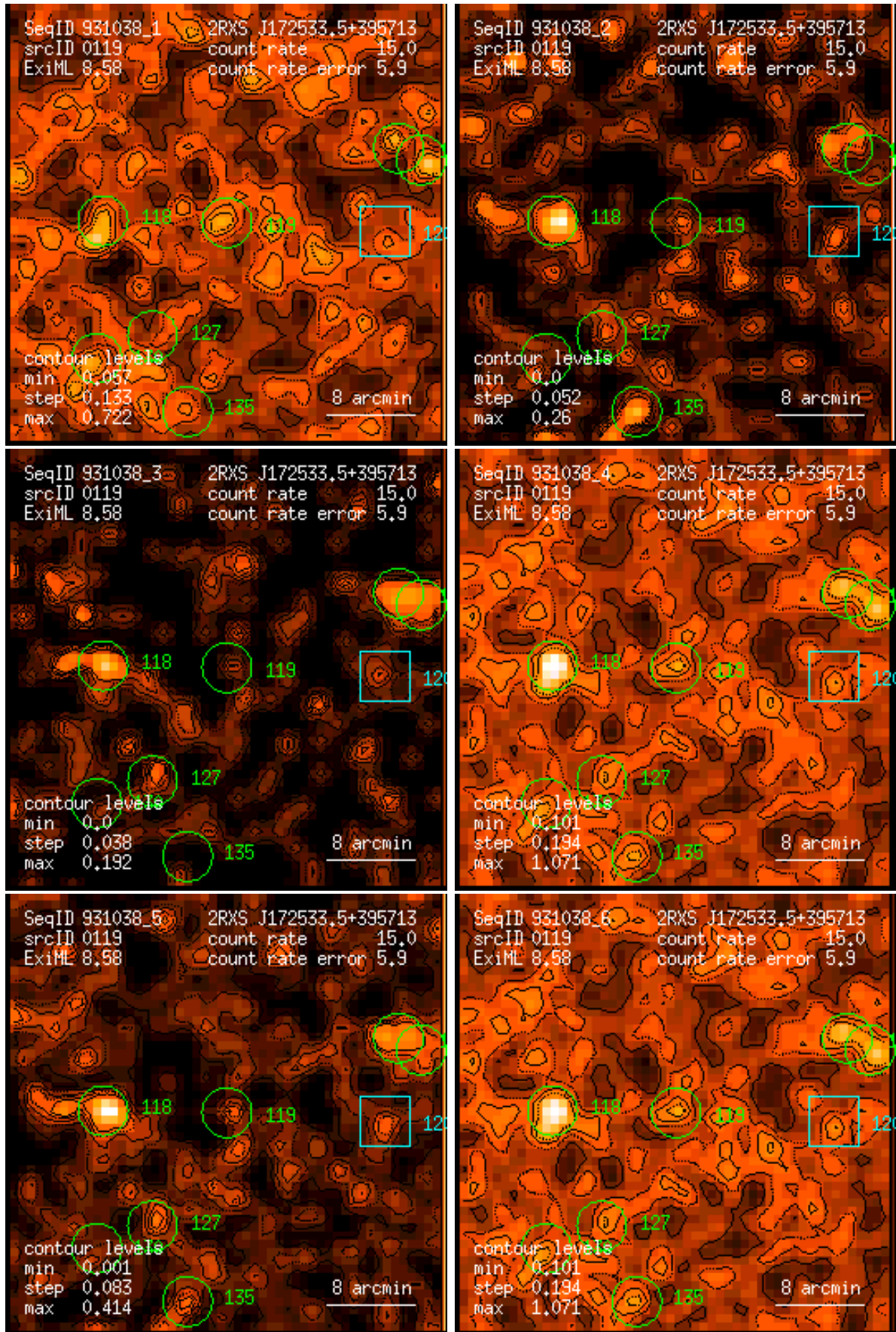
Figure 119: RASS 931038: detection 0119: band rate images, Gaussian filter: (1) PSPC channels 11 – 41, (2) 52 – 90, (3) 91 – 201, (4) 11 – 235, (5) 52 – 201, (6) 11 – 201. Broad band rates in counts/ks. Band rate contour levels in counts/ks/arcmin 2 .
