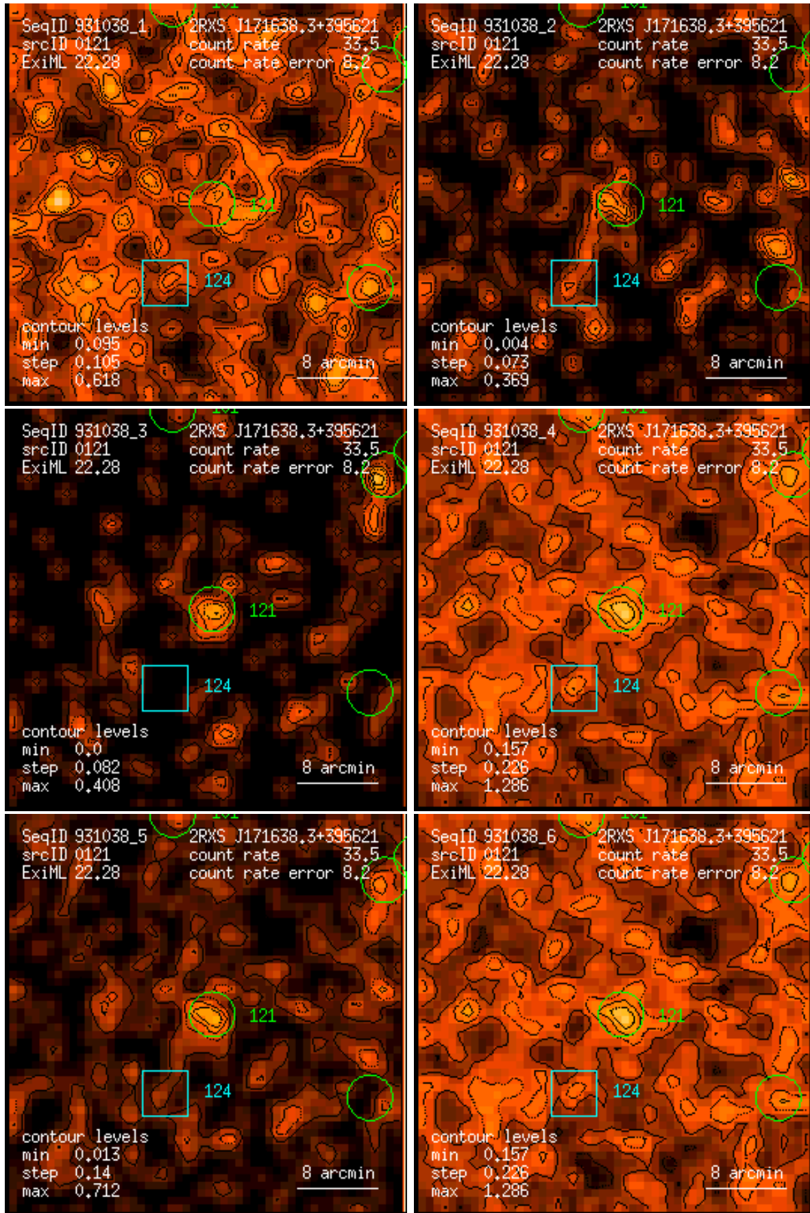
Figure 121: RASS 931038: detection 0121: band rate images, Gaussian filter: (1) PSPC channels 11 – 41, (2) 52 – 90, (3) 91 – 201, (4) 11 – 235, (5) 52 – 201, (6) 11 – 201. Broad band rates in counts/ks. Band rate contour levels in counts/ks/arcmin 2 .
