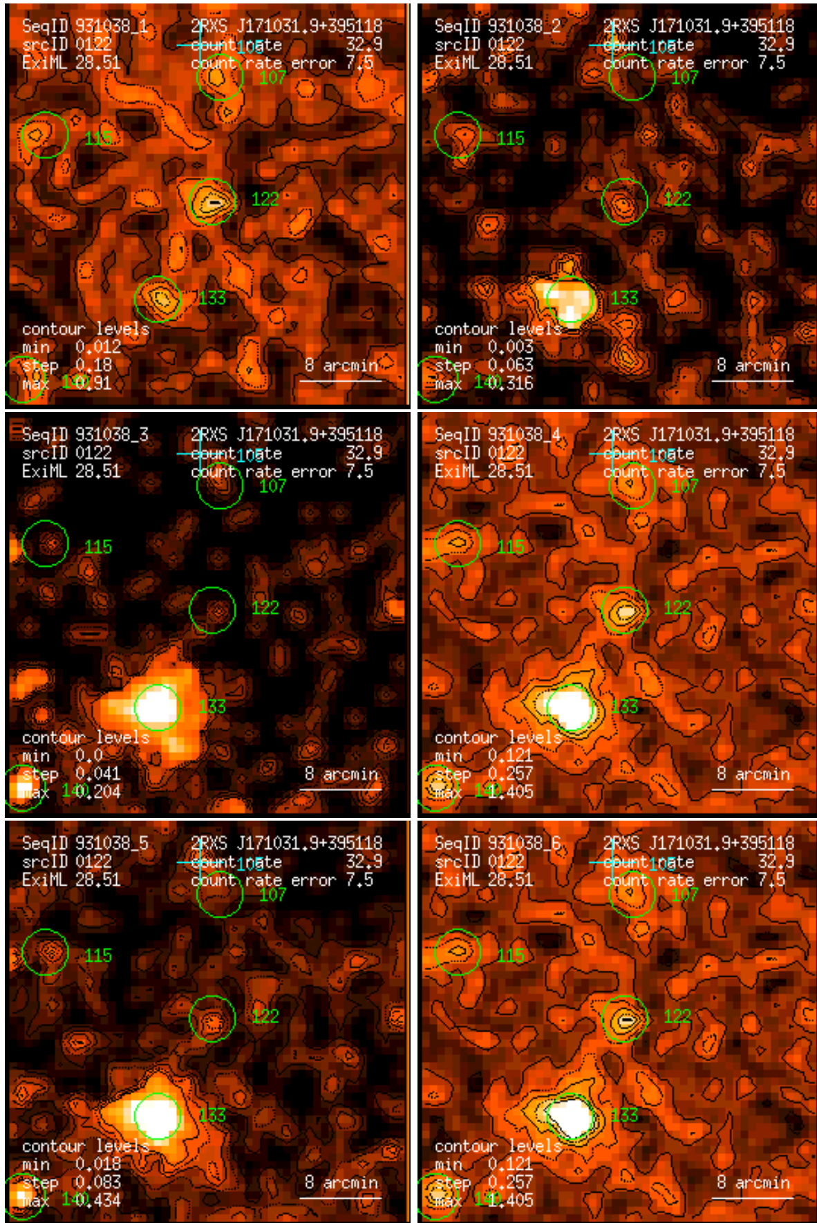
Figure 122: RASS 931038: detection 0122: band rate images, Gaussian filter: (1) PSPC channels 11 – 41, (2) 52 – 90, (3) 91 – 201, (4) 11 – 235, (5) 52 – 201, (6) 11 – 201. Broad band rates in counts/ks. Band rate contour levels in counts/ks/arcmin 2 .
