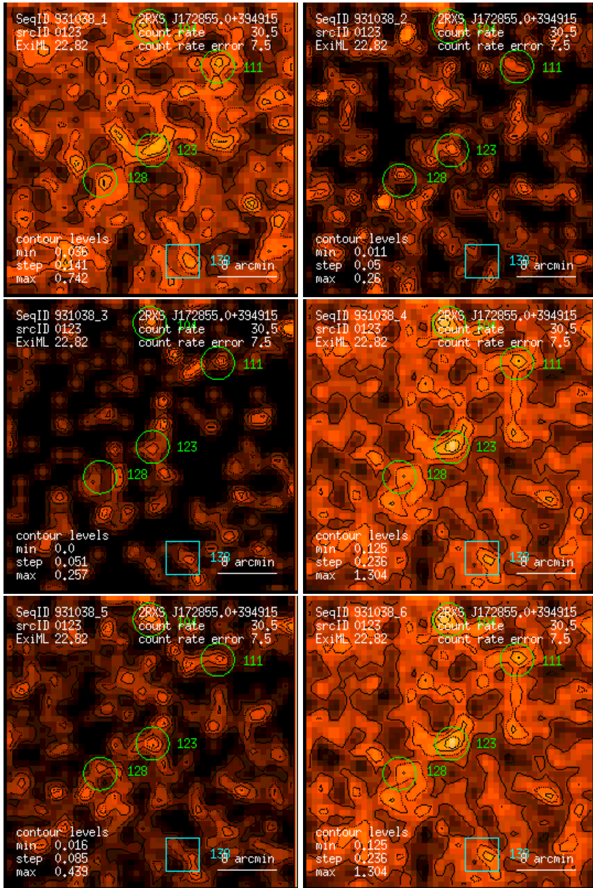
Figure 123: RASS 931038: detection 0123: band rate images, Gaussian filter: (1) PSPC channels 11 – 41, (2) 52 – 90, (3) 91 – 201, (4) 11 – 235, (5) 52 – 201, (6) 11 – 201. Broad band rates in counts/ks. Band rate contour levels in counts/ks/arcmin 2 .
