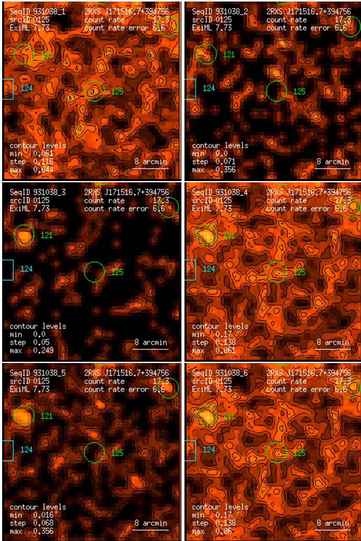
Figure 125: RASS 931038: detection 0125: band rate images, Gaussian filter: (1) PSPC channels 11 – 41, (2) 52 – 90, (3) 91 – 201, (4) 11 – 235, (5) 52 – 201, (6) 11 – 201. Broad band rates in counts/ks. Band rate contour levels in counts/ks/arcmin 2 .
