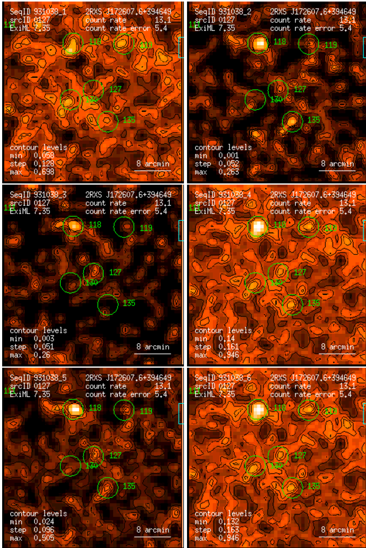
Figure 127: RASS 931038: detection 0127: band rate images, Gaussian filter: (1) PSPC channels 11 – 41, (2) 52 – 90, (3) 91 – 201, (4) 11 – 235, (5) 52 – 201, (6) 11 – 201. Broad band rates in counts/ks. Band rate contour levels in counts/ks/arcmin 2 .
