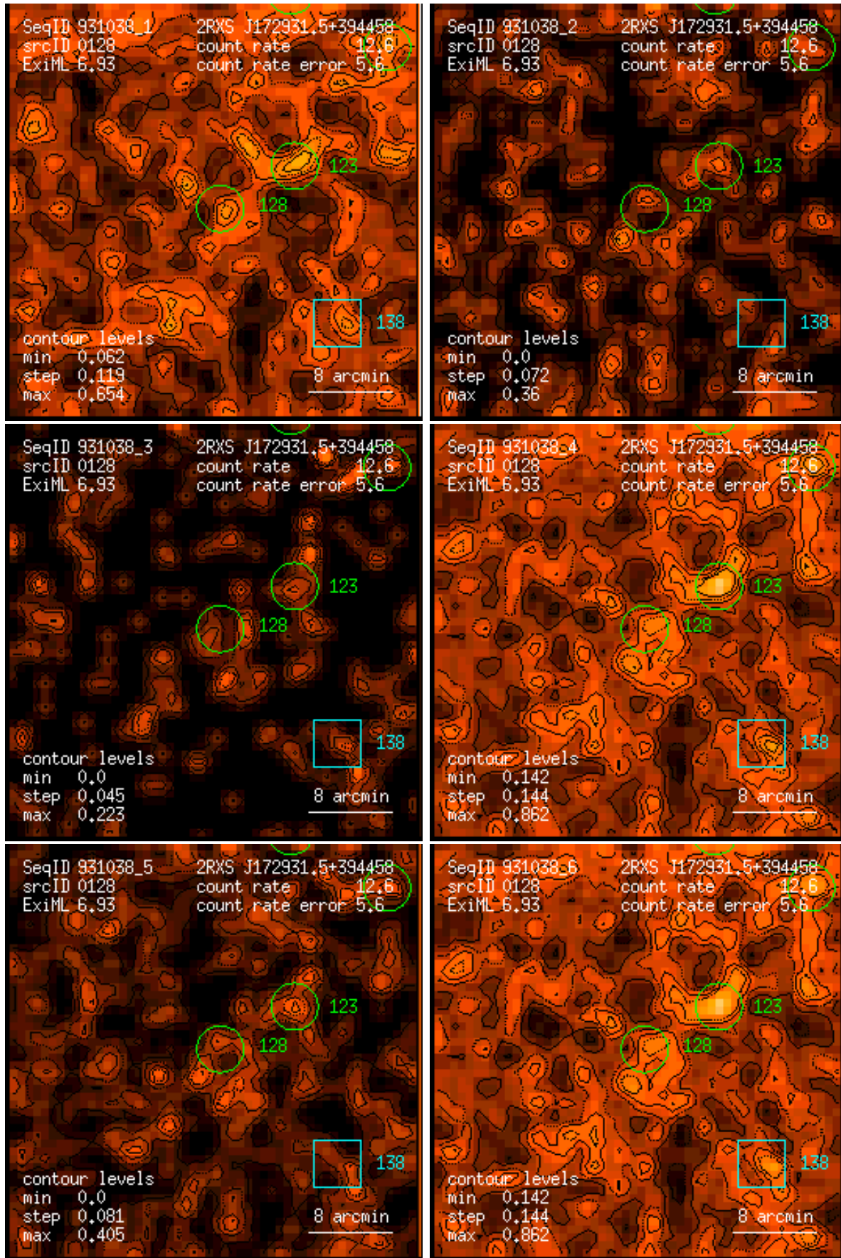
Figure 128: RASS 931038: detection 0128: band rate images, Gaussian filter: (1) PSPC channels 11 – 41, (2) 52 – 90, (3) 91 – 201, (4) 11 – 235, (5) 52 – 201, (6) 11 – 201. Broad band rates in counts/ks. Band rate contour levels in counts/ks/arcmin 2 .
