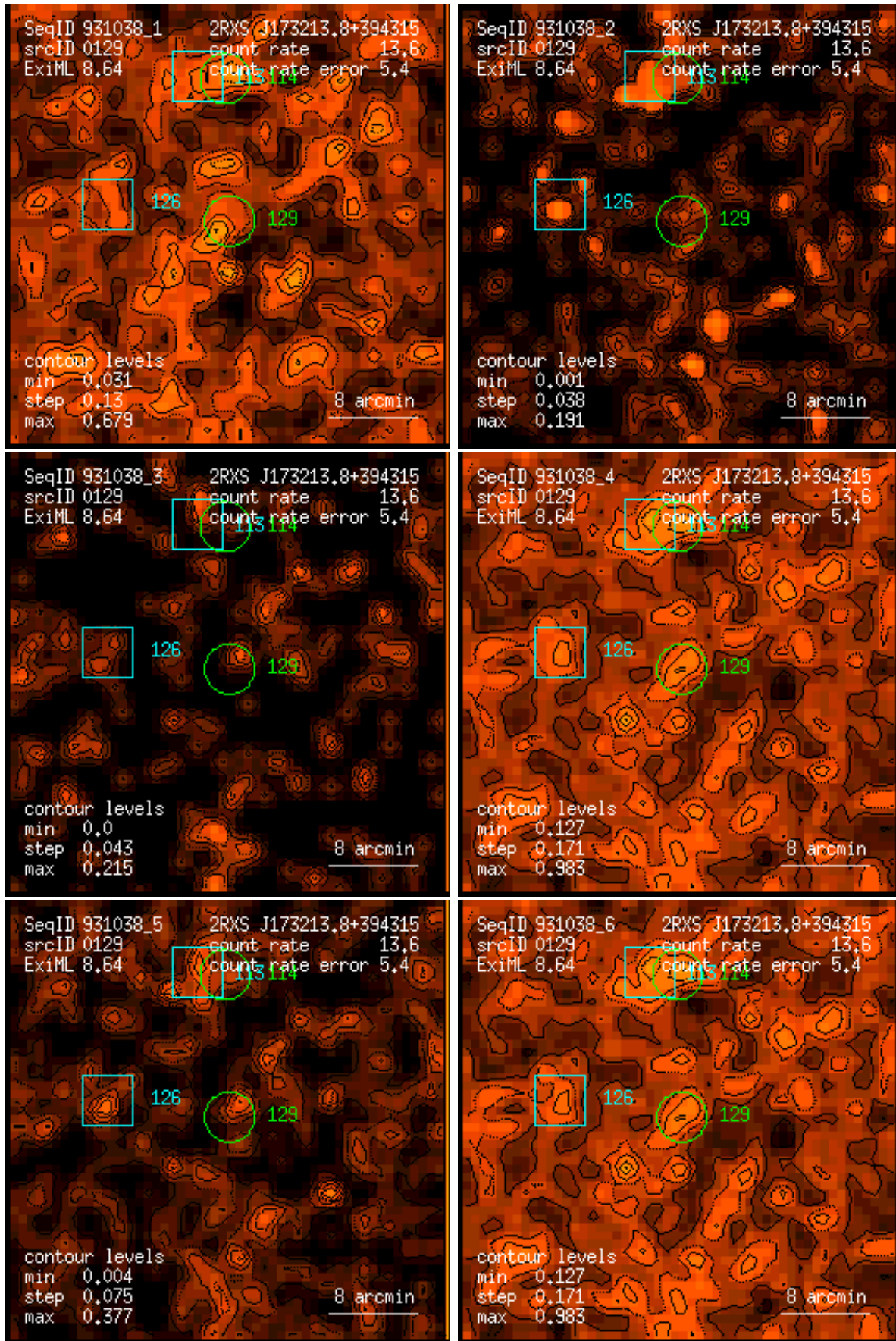
Figure 129: RASS 931038: detection 0129: band rate images, Gaussian filter: (1) PSPC channels 11 – 41, (2) 52 – 90, (3) 91 – 201, (4) 11 – 235, (5) 52 – 201, (6) 11 – 201. Broad band rates in counts/ks. Band rate contour levels in counts/ks/arcmin 2 .
