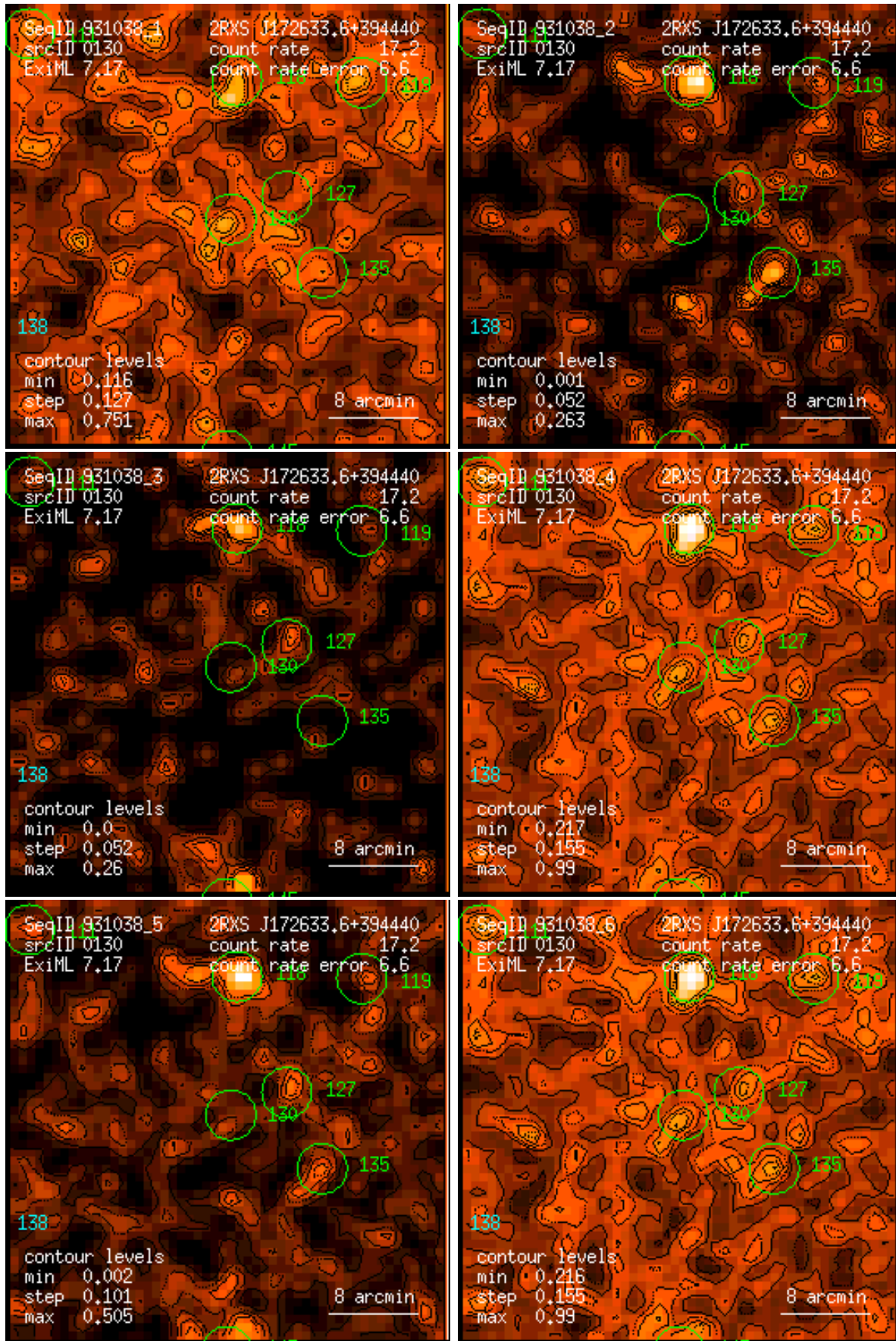
Figure 130: RASS 931038: detection 0130: band rate images, Gaussian filter: (1) PSPC channels 11 – 41, (2) 52 – 90, (3) 91 – 201, (4) 11 – 235, (5) 52 – 201, (6) 11 – 201. Broad band rates in counts/ks. Band rate contour levels in counts/ks/arcmin 2 .
