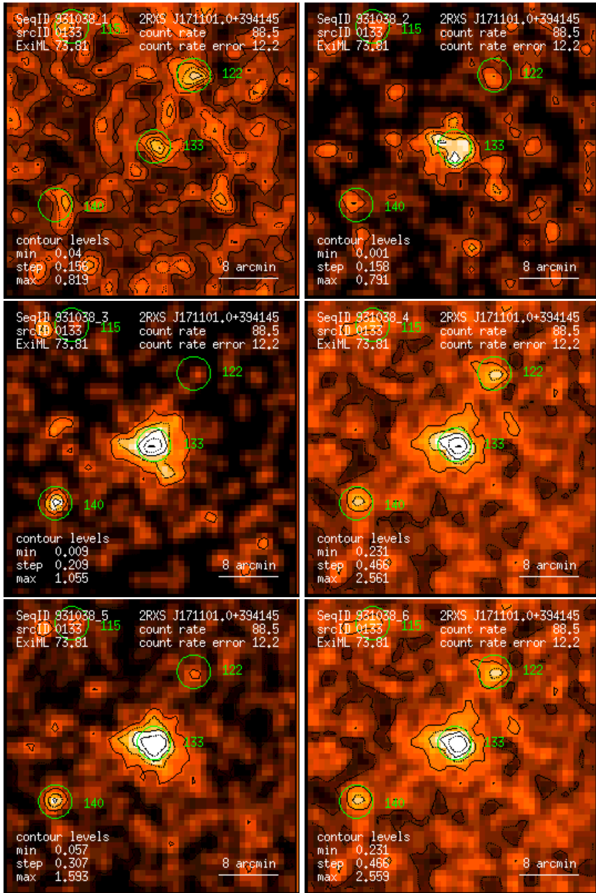
Figure 133: RASS 931038: detection 0133: band rate images, Gaussian filter: (1) PSPC channels 11 – 41, (2) 52 – 90, (3) 91 – 201, (4) 11 – 235, (5) 52 – 201, (6) 11 – 201. Broad band rates in counts/ks. Band rate contour levels in counts/ks/arcmin 2 .
