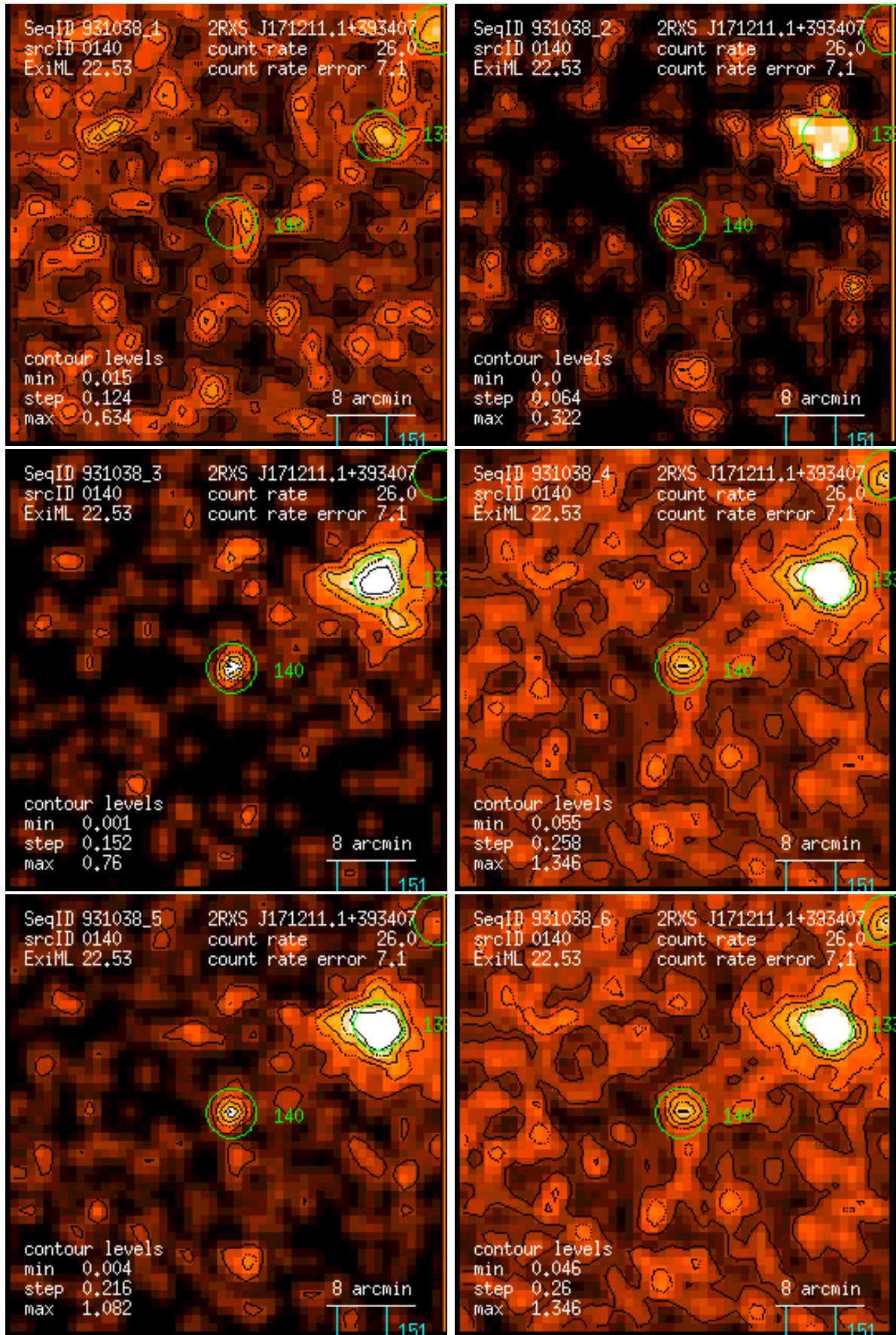
Figure 140: RASS 931038: detection 0140: band rate images, Gaussian filter: (1) PSPC channels 11 – 41, (2) 52 – 90, (3) 91 – 201, (4) 11 – 235, (5) 52 – 201, (6) 11 – 201. Broad band rates in counts/ks. Band rate contour levels in counts/ks/arcmin 2 .
