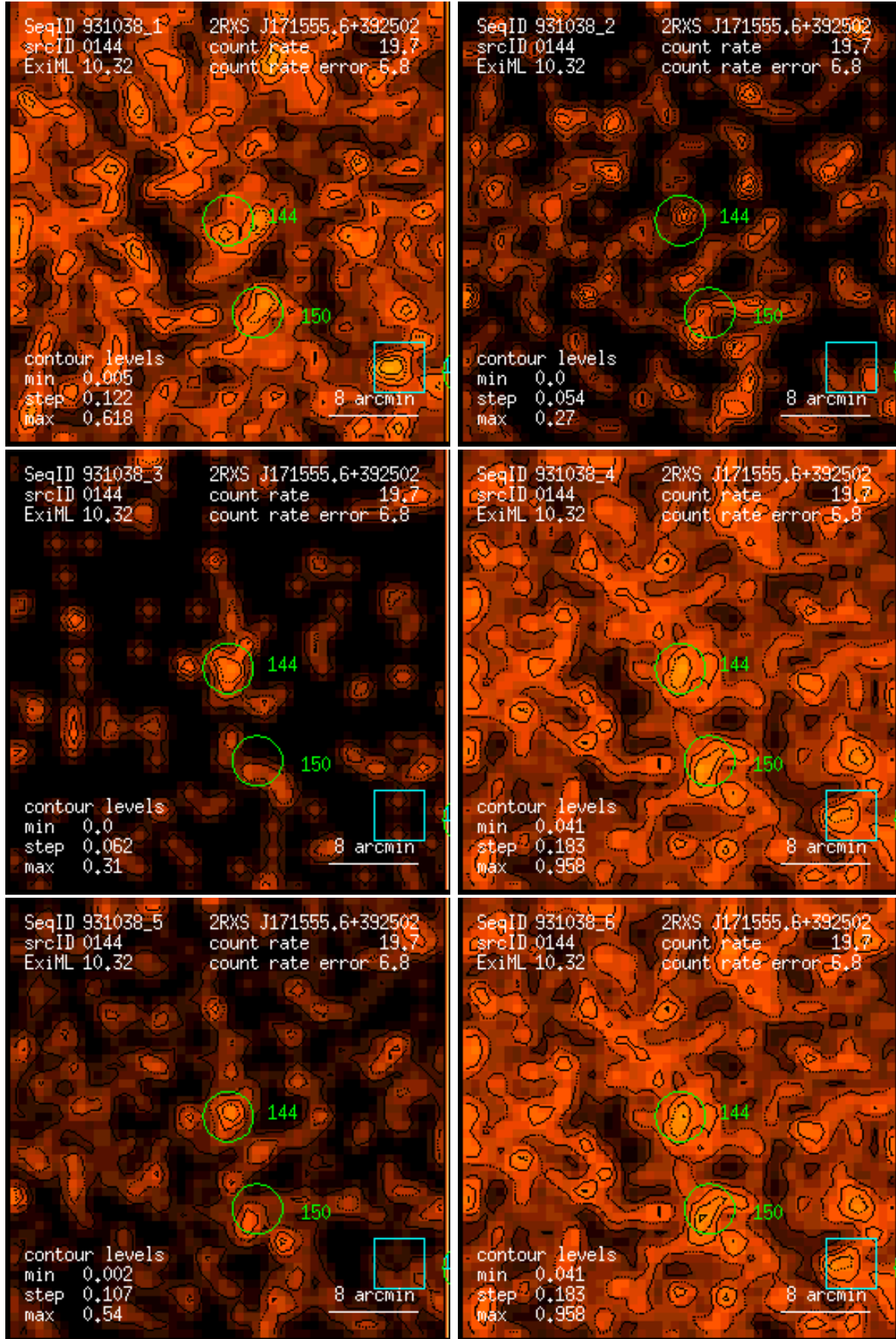
Figure 144: RASS 931038: detection 0144: band rate images, Gaussian filter: (1) PSPC channels 11 – 41, (2) 52 – 90, (3) 91 – 201, (4) 11 – 235, (5) 52 – 201, (6) 11 – 201. Broad band rates in counts/ks. Band rate contour levels in counts/ks/arcmin 2 .
