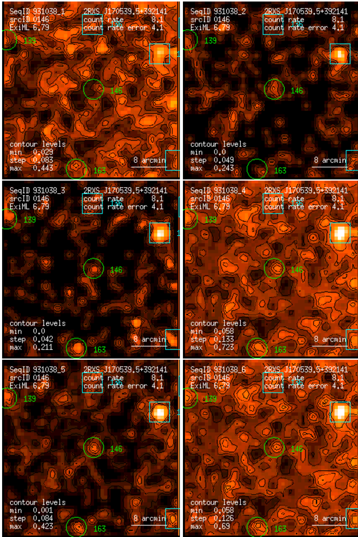
Figure 146: RASS 931038: detection 0146: band rate images, Gaussian filter: (1) PSPC channels 11 – 41, (2) 52 – 90, (3) 91 – 201, (4) 11 – 235, (5) 52 – 201, (6) 11 – 201. Broad band rates in counts/ks. Band rate contour levels in counts/ks/arcmin 2 .
