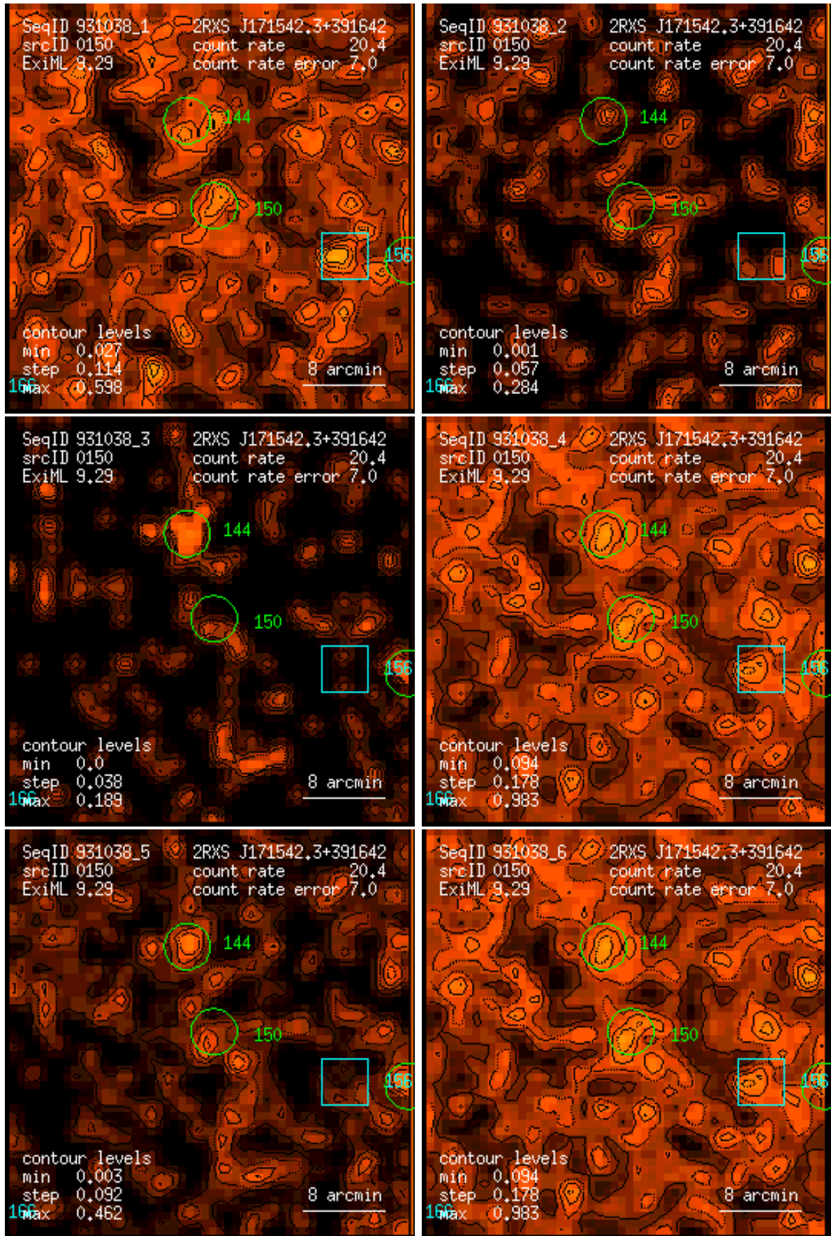
Figure 150: RASS 931038: detection 0150: band rate images, Gaussian filter: (1) PSPC channels 11 – 41, (2) 52 – 90, (3) 91 – 201, (4) 11 – 235, (5) 52 – 201, (6) 11 – 201. Broad band rates in counts/ks. Band rate contour levels in counts/ks/arcmin 2 .
