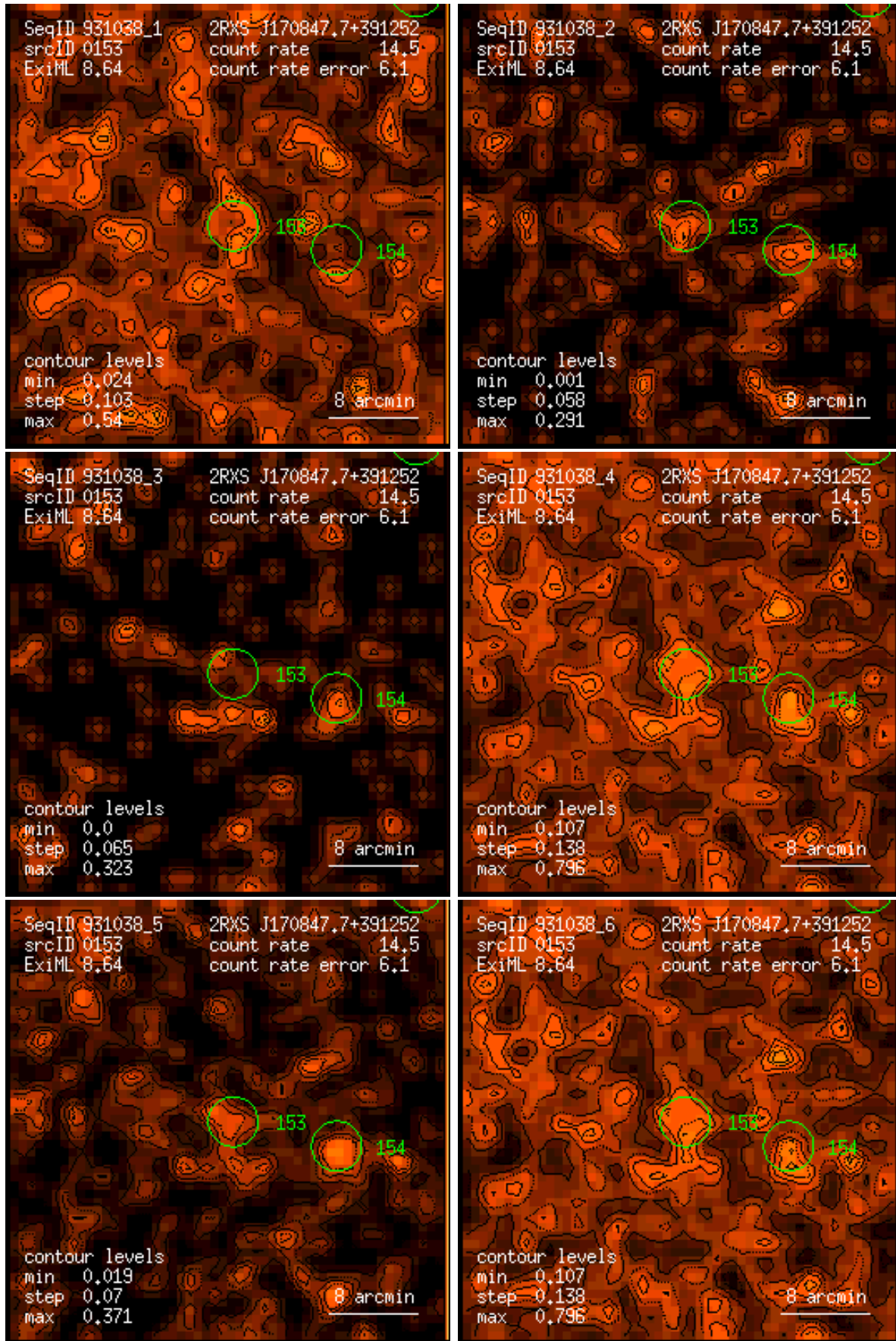
Figure 153: RASS 931038: detection 0153: band rate images, Gaussian filter: (1) PSPC channels 11 – 41, (2) 52 – 90, (3) 91 – 201, (4) 11 – 235, (5) 52 – 201, (6) 11 – 201. Broad band rates in counts/ks. Band rate contour levels in counts/ks/arcmin 2 .
