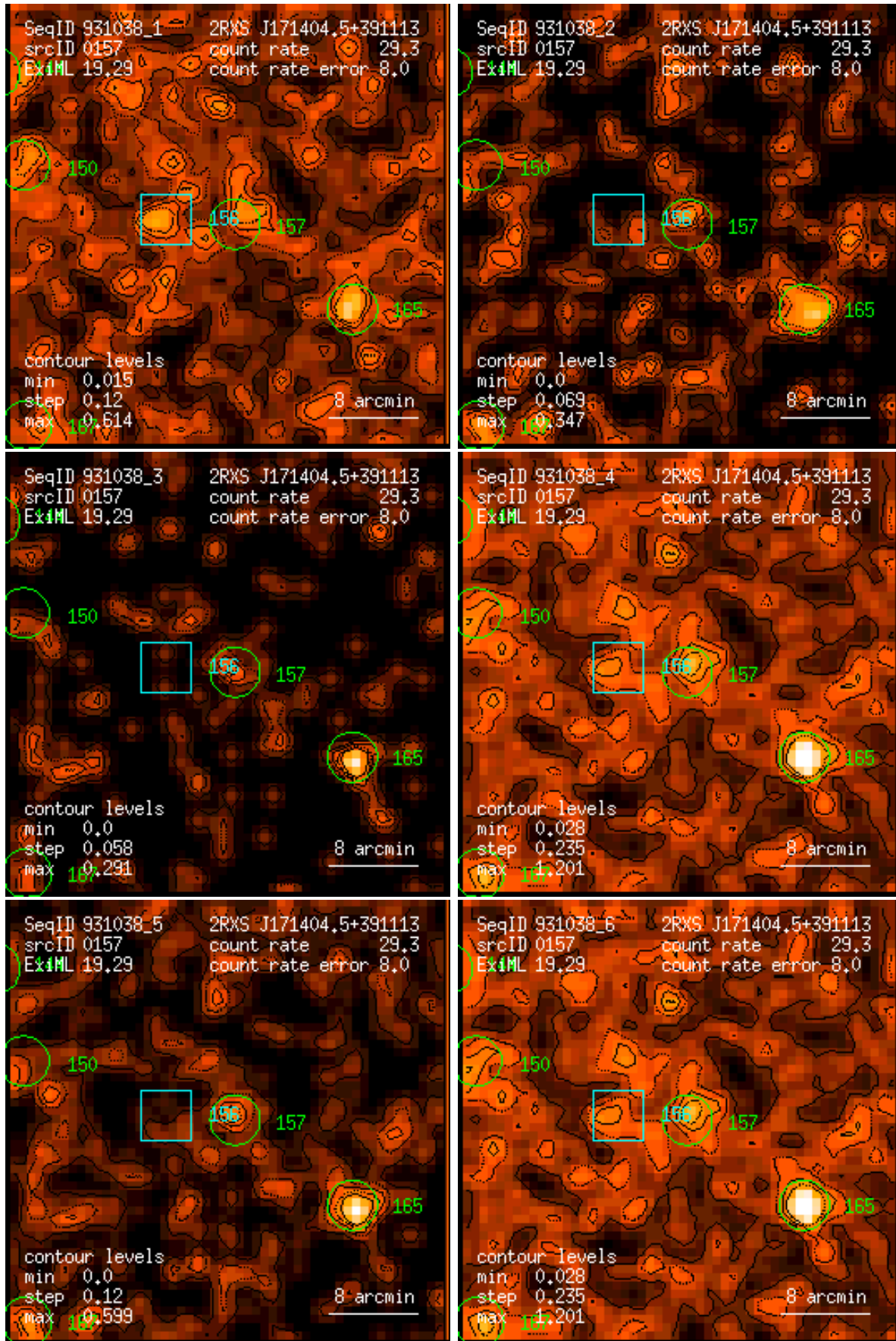
Figure 157: RASS 931038: detection 0157: band rate images, Gaussian filter: (1) PSPC channels 11 – 41, (2) 52 – 90, (3) 91 – 201, (4) 11 – 235, (5) 52 – 201, (6) 11 – 201. Broad band rates in counts/ks. Band rate contour levels in counts/ks/arcmin 2 .
