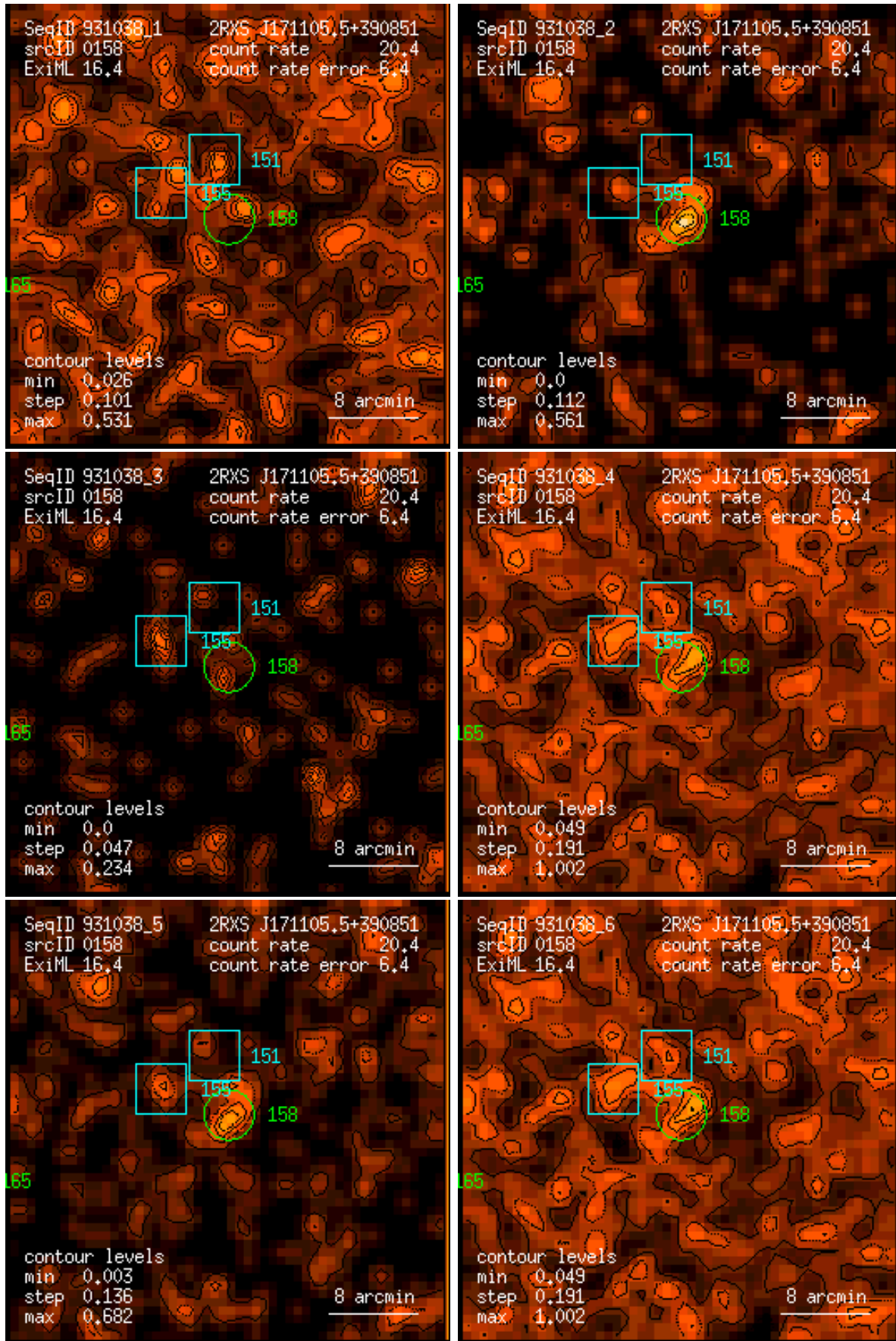
Figure 158: RASS 931038: detection 0158: band rate images, Gaussian filter: (1) PSPC channels 11 – 41, (2) 52 – 90, (3) 91 – 201, (4) 11 – 235, (5) 52 – 201, (6) 11 – 201. Broad band rates in counts/ks. Band rate contour levels in counts/ks/arcmin 2 .
