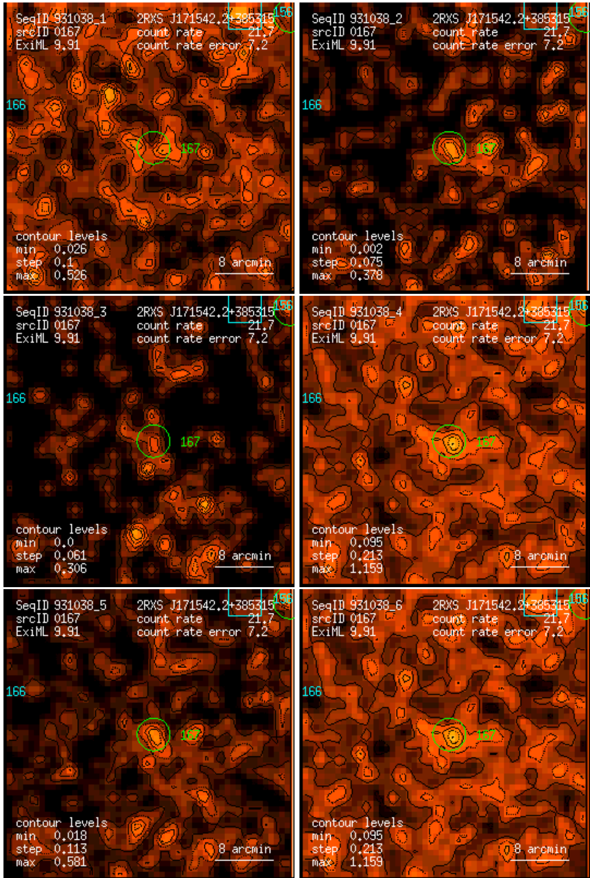
Figure 167: RASS 931038: detection 0167: band rate images, Gaussian filter: (1) PSPC channels 11 – 41, (2) 52 – 90, (3) 91 – 201, (4) 11 – 235, (5) 52 – 201, (6) 11 – 201. Broad band rates in counts/ks. Band rate contour levels in counts/ks/arcmin 2 .
