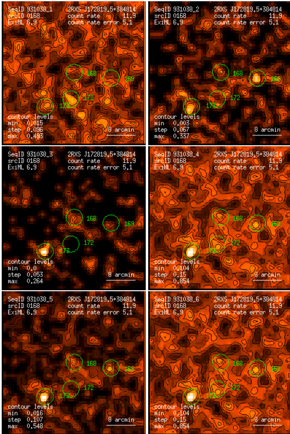
Figure 168: RASS 931038: detection 0168: band rate images, Gaussian filter: (1) PSPC channels 11 – 41, (2) 52 – 90, (3) 91 – 201, (4) 11 – 235, (5) 52 – 201, (6) 11 – 201. Broad band rates in counts/ks. Band rate contour levels in counts/ks/arcmin 2 .
