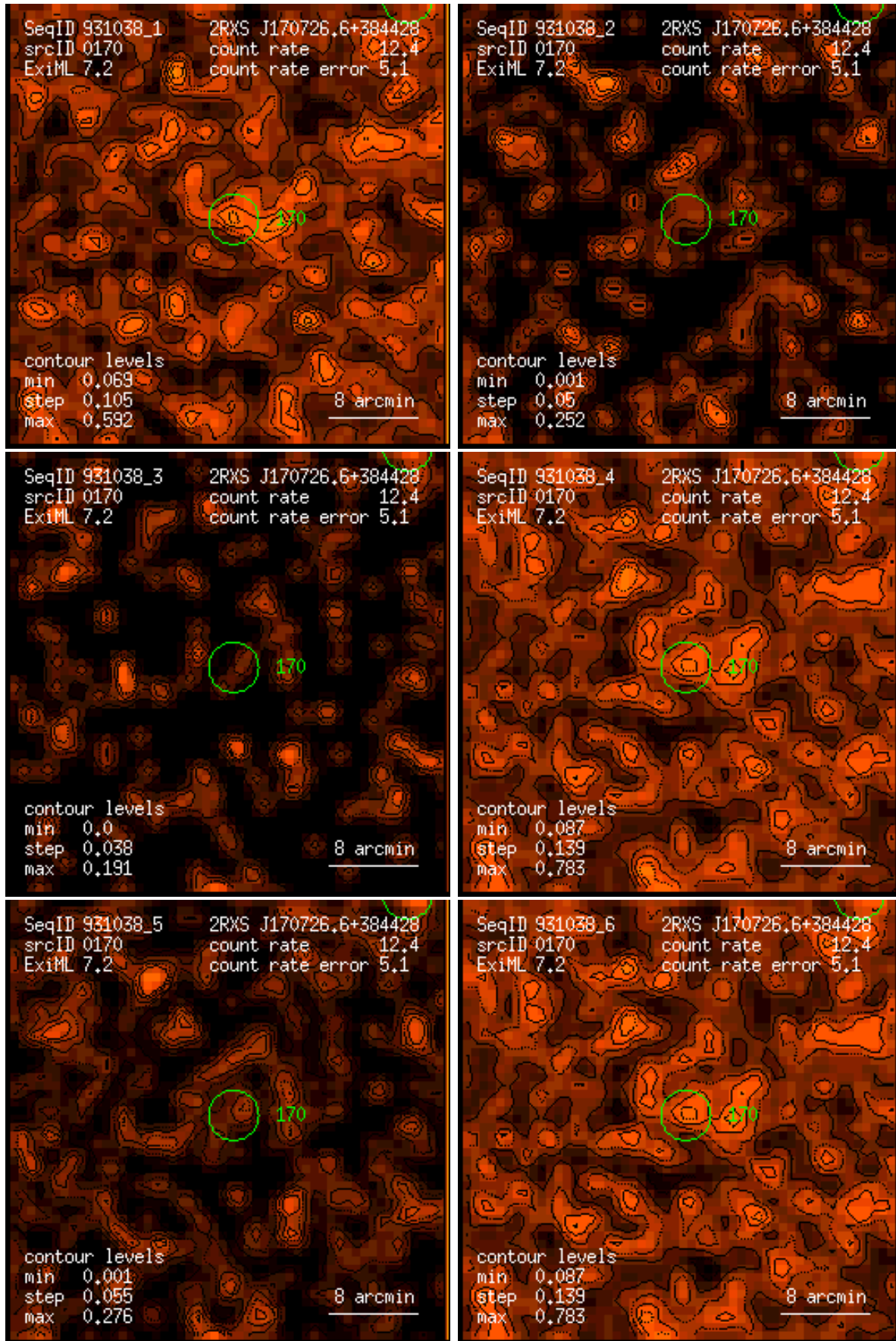
Figure 170: RASS 931038: detection 0170: band rate images, Gaussian filter: (1) PSPC channels 11 – 41, (2) 52 – 90, (3) 91 – 201, (4) 11 – 235, (5) 52 – 201, (6) 11 – 201. Broad band rates in counts/ks. Band rate contour levels in counts/ks/arcmin 2 .
