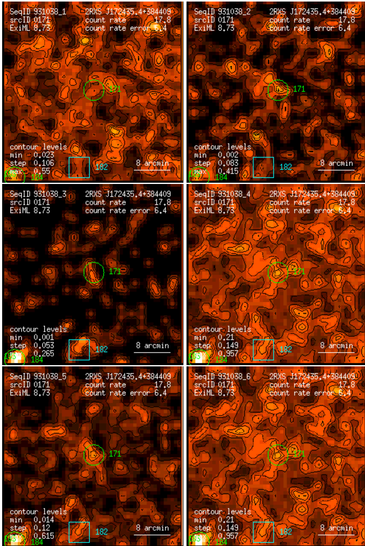
Figure 171: RASS 931038: detection 0171: band rate images, Gaussian filter: (1) PSPC channels 11 – 41, (2) 52 – 90, (3) 91 – 201, (4) 11 – 235, (5) 52 – 201, (6) 11 – 201. Broad band rates in counts/ks. Band rate contour levels in counts/ks/arcmin 2 .
