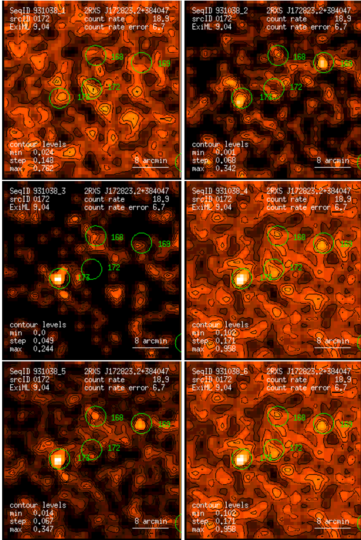
Figure 172: RASS 931038: detection 0172: band rate images, Gaussian filter: (1) PSPC channels 11 – 41, (2) 52 – 90, (3) 91 – 201, (4) 11 – 235, (5) 52 – 201, (6) 11 – 201. Broad band rates in counts/ks. Band rate contour levels in counts/ks/arcmin 2 .
