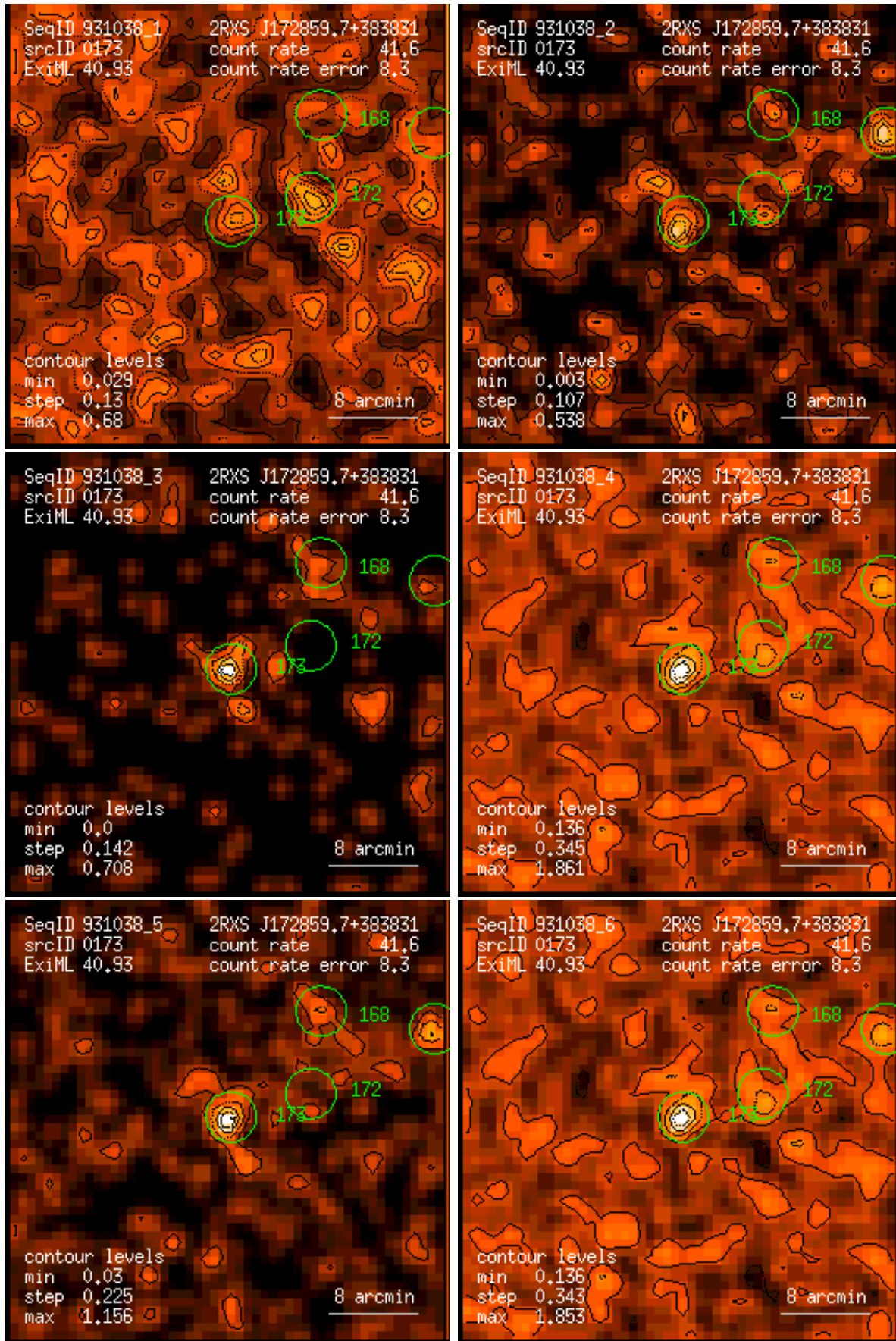
Figure 173: RASS 931038: detection 0173: band rate images, Gaussian filter: (1) PSPC channels 11 – 41, (2) 52 – 90, (3) 91 – 201, (4) 11 – 235, (5) 52 – 201, (6) 11 – 201. Broad band rates in counts/ks. Band rate contour levels in counts/ks/arcmin 2 .
