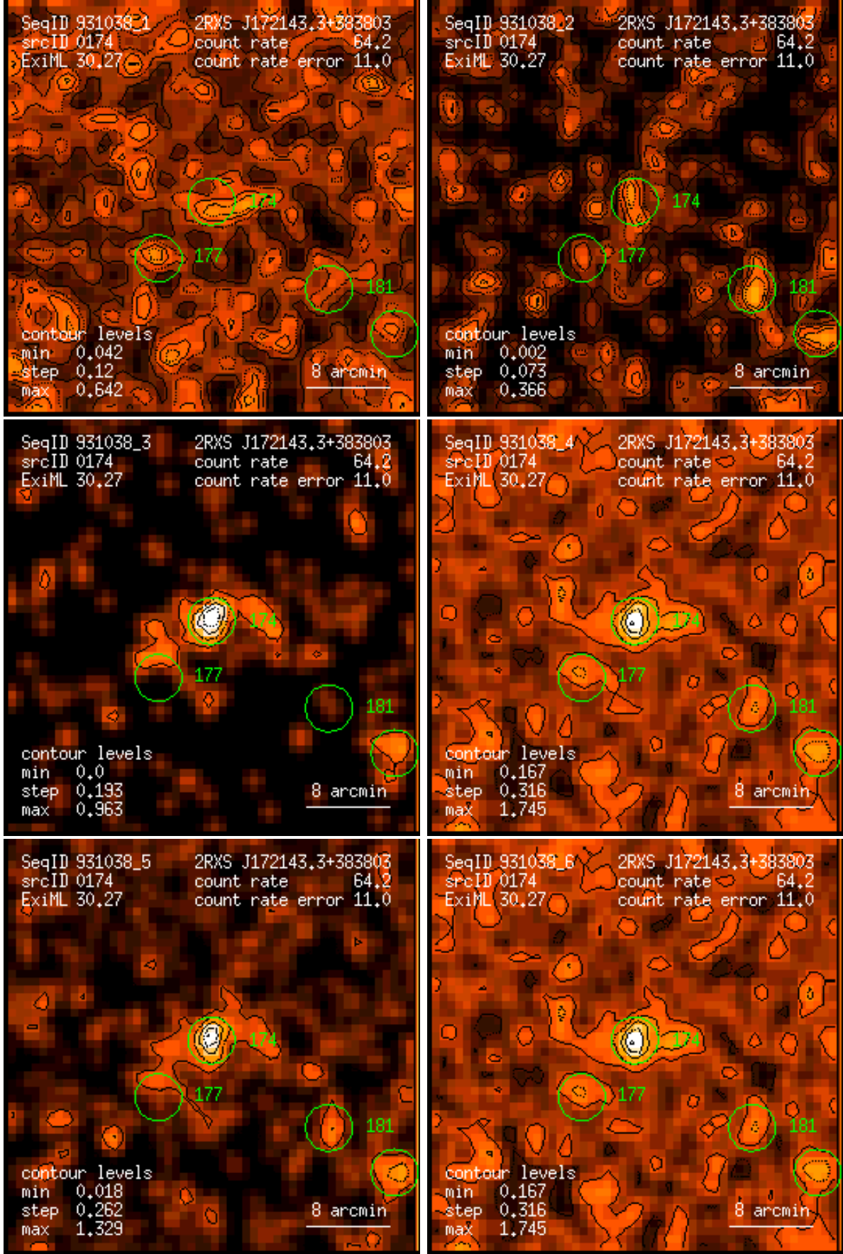
Figure 174: RASS 931038: detection 0174: band rate images, Gaussian filter: (1) PSPC channels 11 – 41, (2) 52 – 90, (3) 91 – 201, (4) 11 – 235, (5) 52 – 201, (6) 11 – 201. Broad band rates in counts/ks. Band rate contour levels in counts/ks/arcmin 2 .
