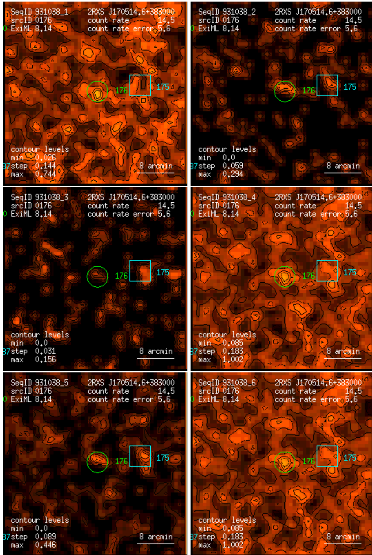
Figure 176: RASS 931038: detection 0176: band rate images, Gaussian filter: (1) PSPC channels 11 – 41, (2) 52 – 90, (3) 91 – 201, (4) 11 – 235, (5) 52 – 201, (6) 11 – 201. Broad band rates in counts/ks. Band rate contour levels in counts/ks/arcmin 2 .
