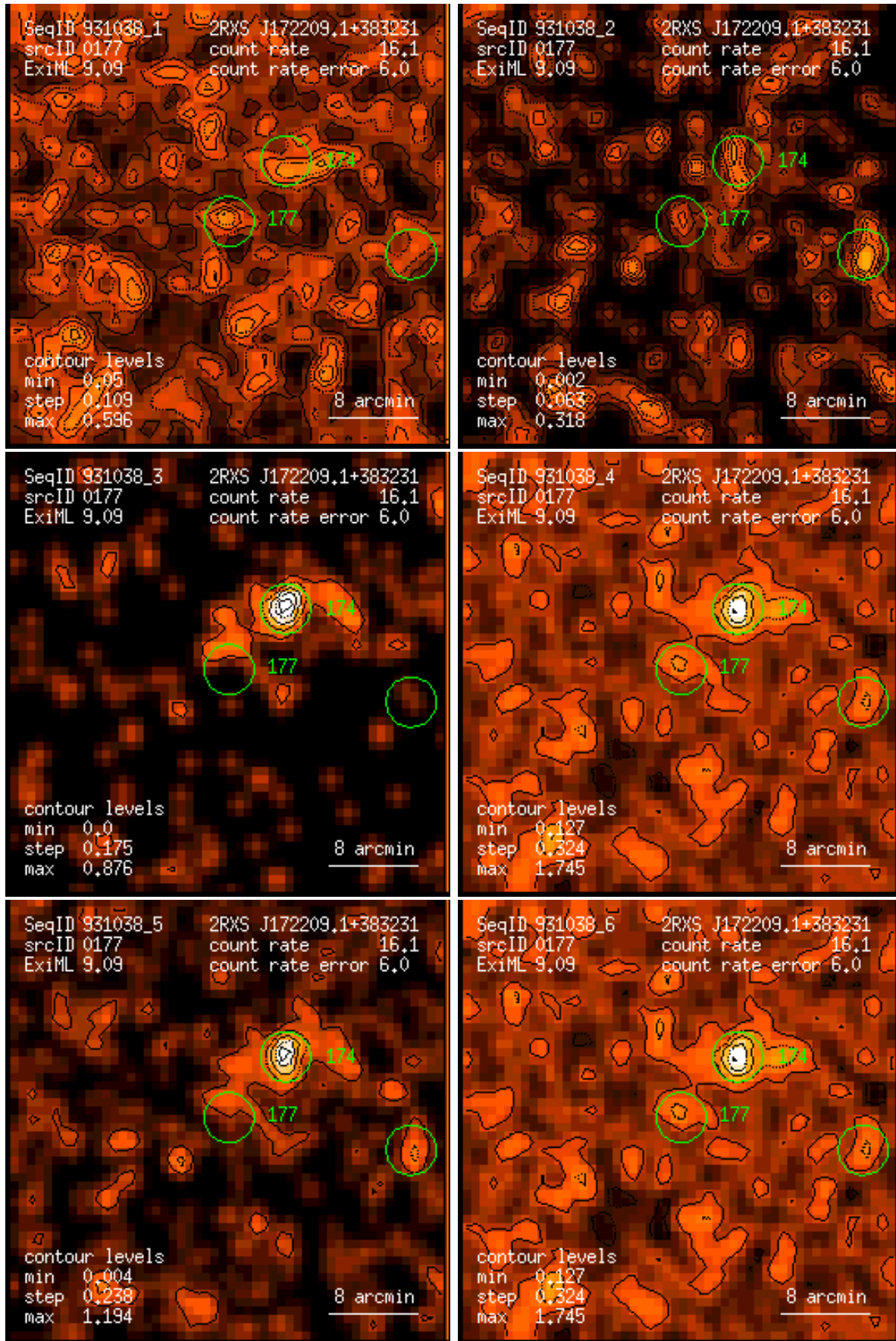
Figure 177: RASS 931038: detection 0177: band rate images, Gaussian filter: (1) PSPC channels 11 – 41, (2) 52 – 90, (3) 91 – 201, (4) 11 – 235, (5) 52 – 201, (6) 11 – 201. Broad band rates in counts/ks. Band rate contour levels in counts/ks/arcmin 2 .
