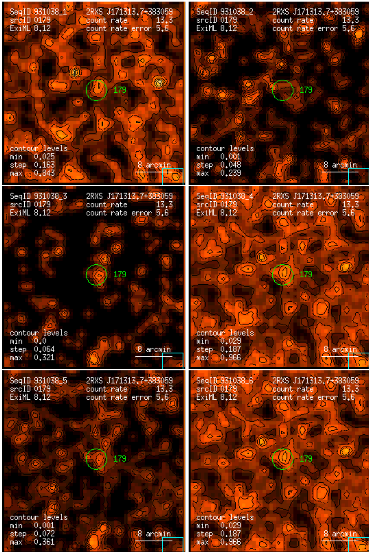
Figure 179: RASS 931038: detection 0179: band rate images, Gaussian filter: (1) PSPC channels 11 – 41, (2) 52 – 90, (3) 91 – 201, (4) 11 – 235, (5) 52 – 201, (6) 11 – 201. Broad band rates in counts/ks. Band rate contour levels in counts/ks/arcmin 2 .
