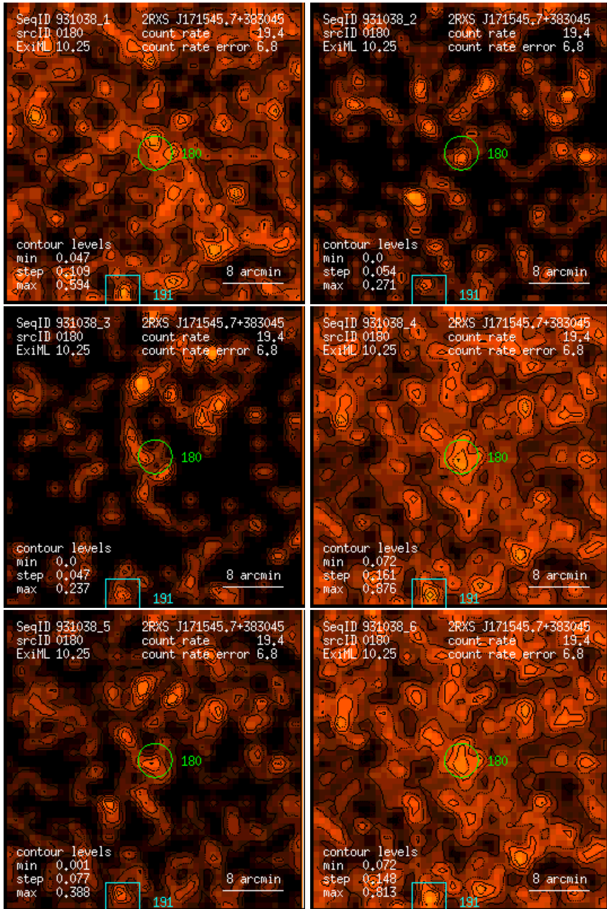
Figure 180: RASS 931038: detection 0180: band rate images, Gaussian filter: (1) PSPC channels 11 – 41, (2) 52 – 90, (3) 91 – 201, (4) 11 – 235, (5) 52 – 201, (6) 11 – 201. Broad band rates in counts/ks. Band rate contour levels in counts/ks/arcmin 2 .
