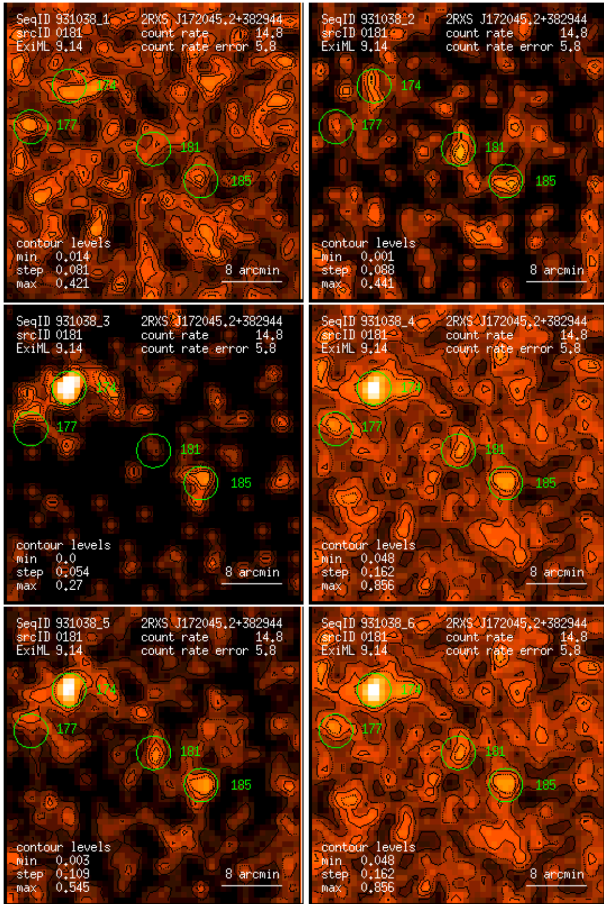
Figure 181: RASS 931038: detection 0181: band rate images, Gaussian filter: (1) PSPC channels 11 – 41, (2) 52 – 90, (3) 91 – 201, (4) 11 – 235, (5) 52 – 201, (6) 11 – 201. Broad band rates in counts/ks. Band rate contour levels in counts/ks/arcmin 2 .
