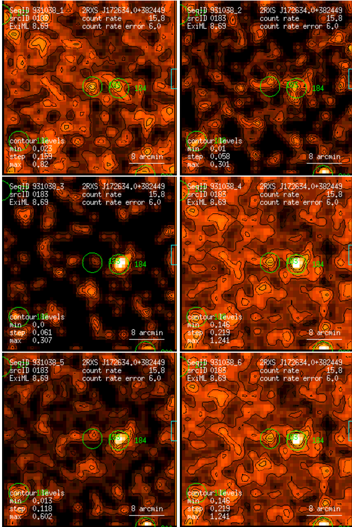
Figure 183: RASS 931038: detection 0183: band rate images, Gaussian filter: (1) PSPC channels 11 – 41, (2) 52 – 90, (3) 91 – 201, (4) 11 – 235, (5) 52 – 201, (6) 11 – 201. Broad band rates in counts/ks. Band rate contour levels in counts/ks/arcmin 2 .
