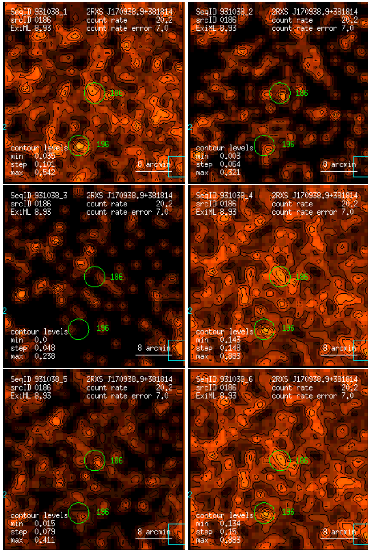
Figure 186: RASS 931038: detection 0186: band rate images, Gaussian filter: (1) PSPC channels 11 – 41, (2) 52 – 90, (3) 91 – 201, (4) 11 – 235, (5) 52 – 201, (6) 11 – 201. Broad band rates in counts/ks. Band rate contour levels in counts/ks/arcmin 2 .
