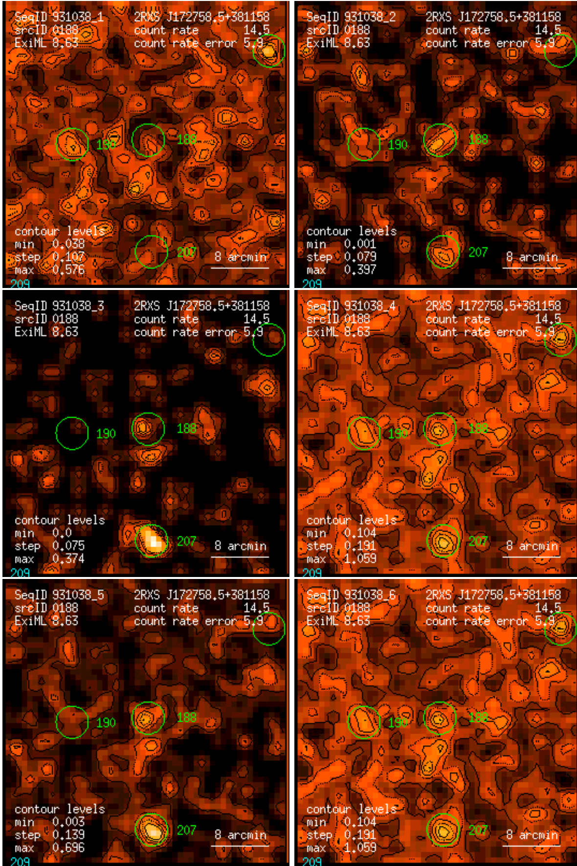
Figure 188: RASS 931038: detection 0188: band rate images, Gaussian filter: (1) PSPC channels 11 – 41, (2) 52 – 90, (3) 91 – 201, (4) 11 – 235, (5) 52 – 201, (6) 11 – 201. Broad band rates in counts/ks. Band rate contour levels in counts/ks/arcmin 2 .
