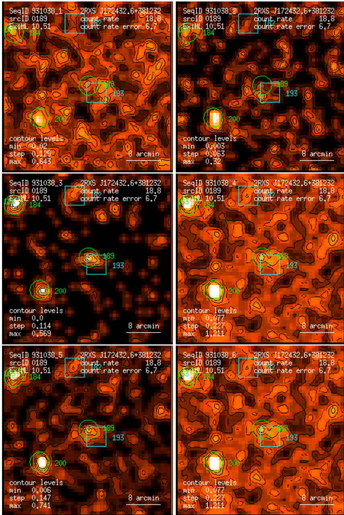
Figure 189: RASS 931038: detection 0189: band rate images, Gaussian filter: (1) PSPC channels 11 – 41, (2) 52 – 90, (3) 91 – 201, (4) 11 – 235, (5) 52 – 201, (6) 11 – 201. Broad band rates in counts/ks. Band rate contour levels in counts/ks/arcmin 2 .
