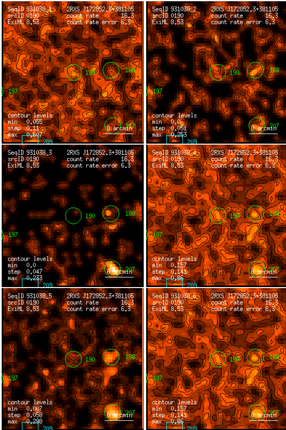
Figure 190: RASS 931038: detection 0190: band rate images, Gaussian filter: (1) PSPC channels 11 – 41, (2) 52 – 90, (3) 91 – 201, (4) 11 – 235, (5) 52 – 201, (6) 11 – 201. Broad band rates in counts/ks. Band rate contour levels in counts/ks/arcmin 2 .
