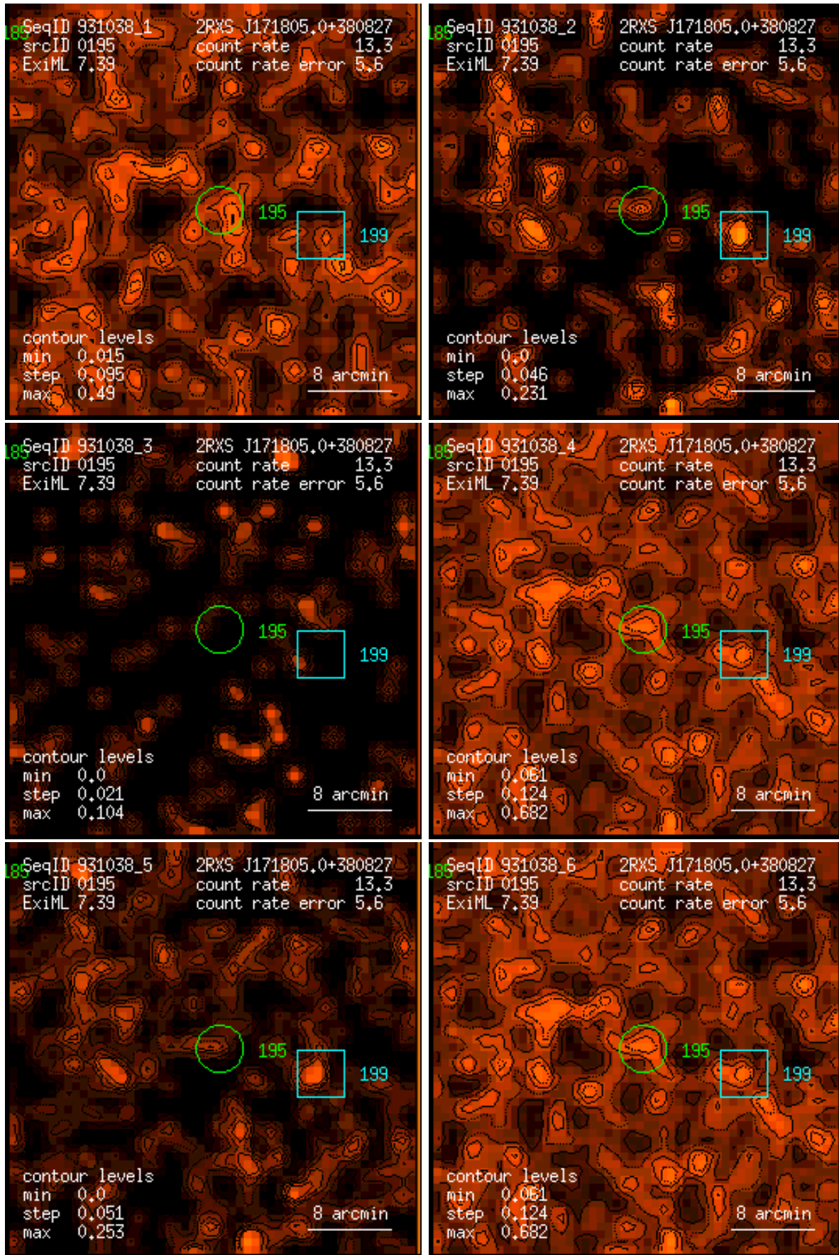
Figure 195: RASS 931038: detection 0195: band rate images, Gaussian filter: (1) PSPC channels 11 – 41, (2) 52 – 90, (3) 91 – 201, (4) 11 – 235, (5) 52 – 201, (6) 11 – 201. Broad band rates in counts/ks. Band rate contour levels in counts/ks/arcmin 2 .
