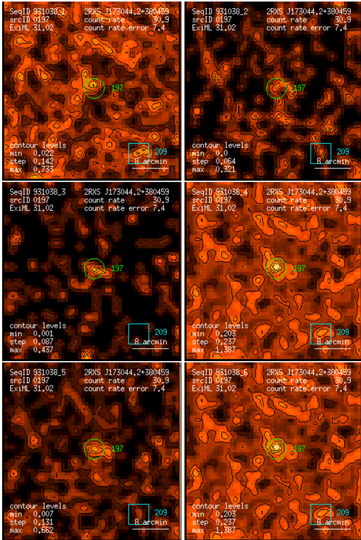
Figure 197: RASS 931038: detection 0197: band rate images, Gaussian filter: (1) PSPC channels 11 – 41, (2) 52 – 90, (3) 91 – 201, (4) 11 – 235, (5) 52 – 201, (6) 11 – 201. Broad band rates in counts/ks. Band rate contour levels in counts/ks/arcmin 2 .
