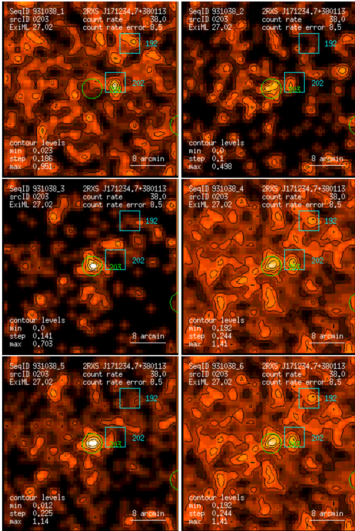
Figure 203: RASS 931038: detection 0203: band rate images, Gaussian filter: (1) PSPC channels 11 – 41, (2) 52 – 90, (3) 91 – 201, (4) 11 – 235, (5) 52 – 201, (6) 11 – 201. Broad band rates in counts/ks. Band rate contour levels in counts/ks/arcmin 2 .
