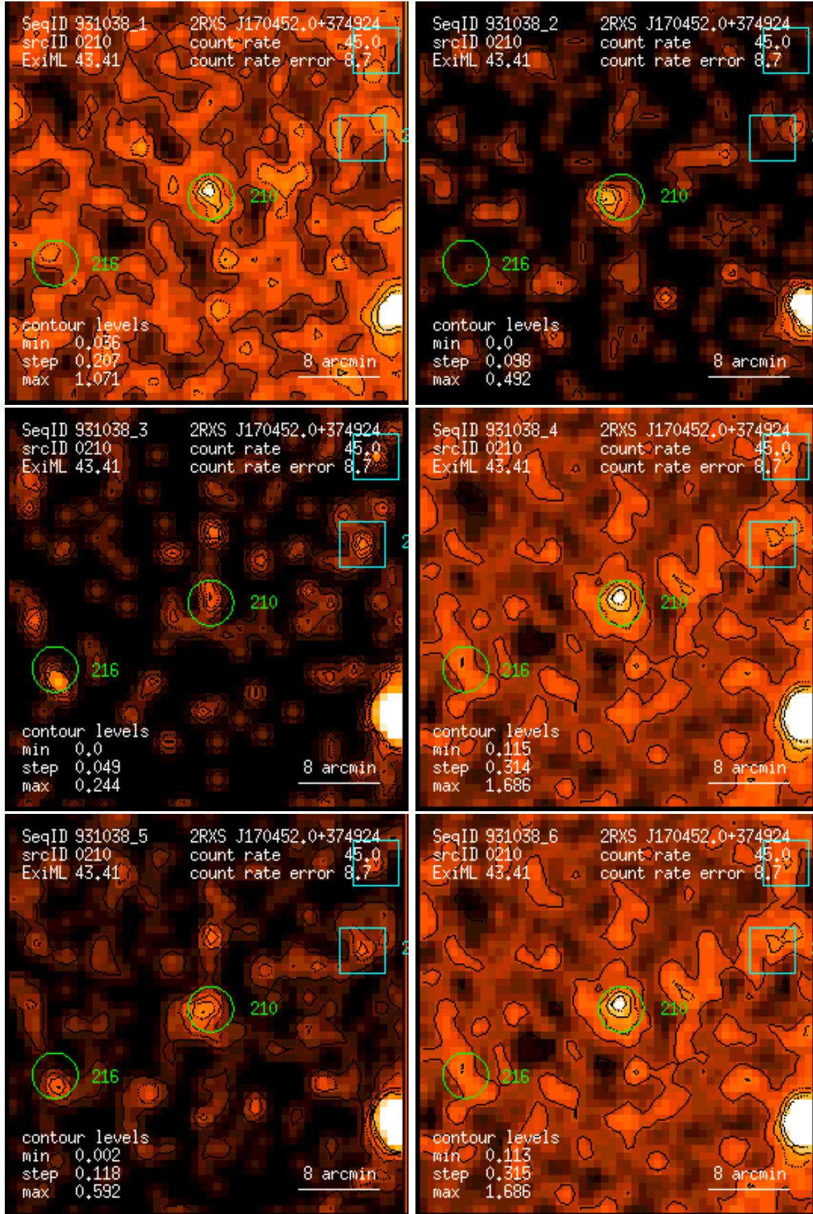
Figure 210: RASS 931038: detection 0210: band rate images, Gaussian filter: (1) PSPC channels 11 – 41, (2) 52 – 90, (3) 91 – 201, (4) 11 – 235, (5) 52 – 201, (6) 11 – 201. Broad band rates in counts/ks. Band rate contour levels in counts/ks/arcmin 2 .
