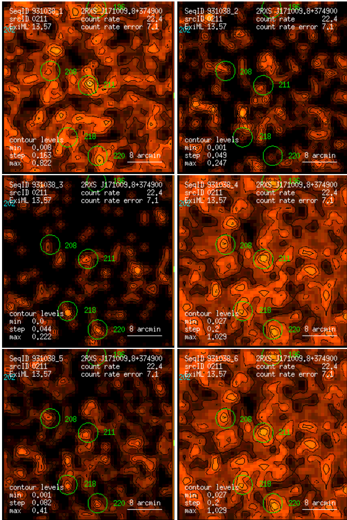
Figure 211: RASS 931038: detection 0211: band rate images, Gaussian filter: (1) PSPC channels 11 – 41, (2) 52 – 90, (3) 91 – 201, (4) 11 – 235, (5) 52 – 201, (6) 11 – 201. Broad band rates in counts/ks. Band rate contour levels in counts/ks/arcmin 2 .
