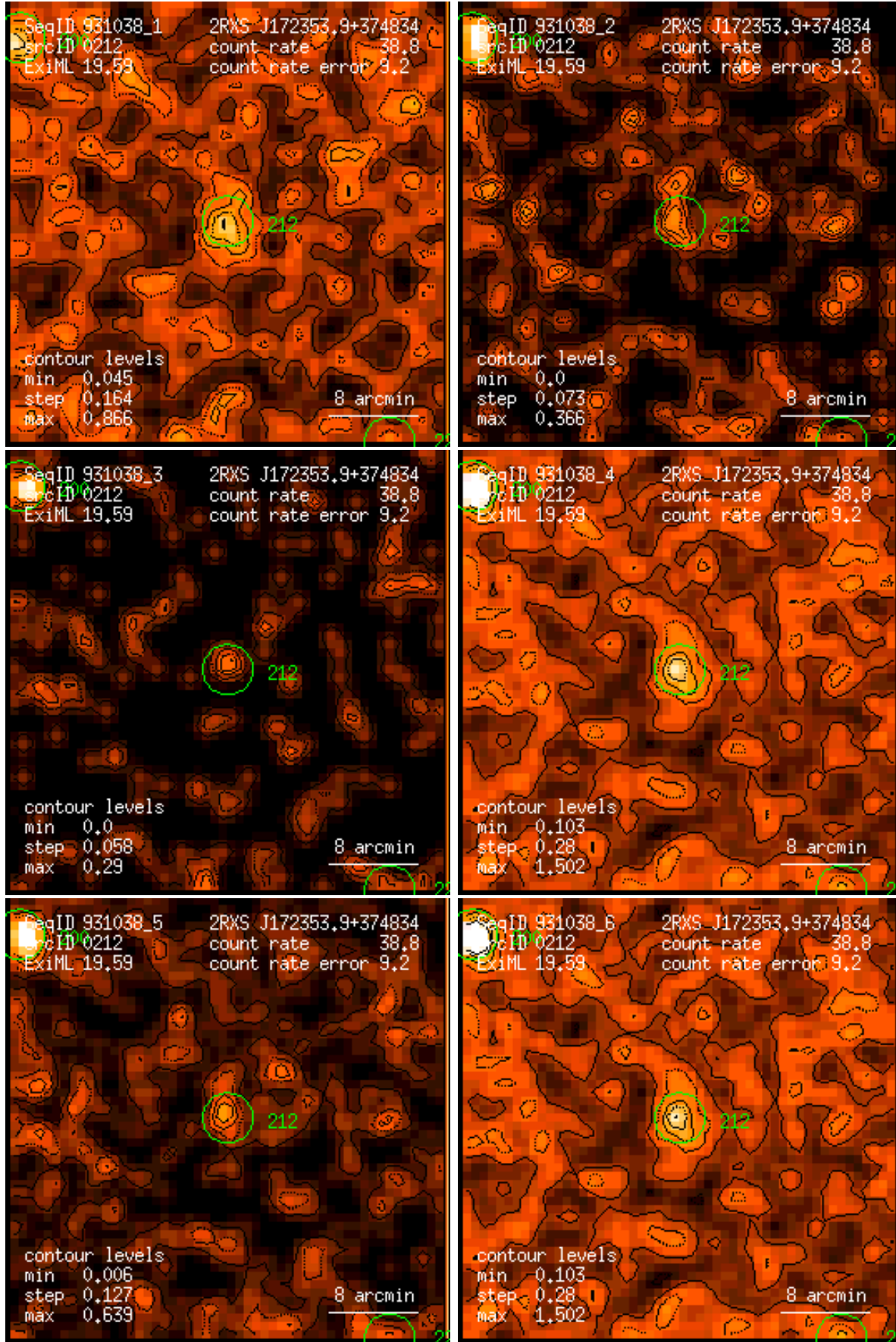
Figure 212: RASS 931038: detection 0212: band rate images, Gaussian filter: (1) PSPC channels 11 – 41, (2) 52 – 90, (3) 91 – 201, (4) 11 – 235, (5) 52 – 201, (6) 11 – 201. Broad band rates in counts/ks. Band rate contour levels in counts/ks/arcmin 2 .
