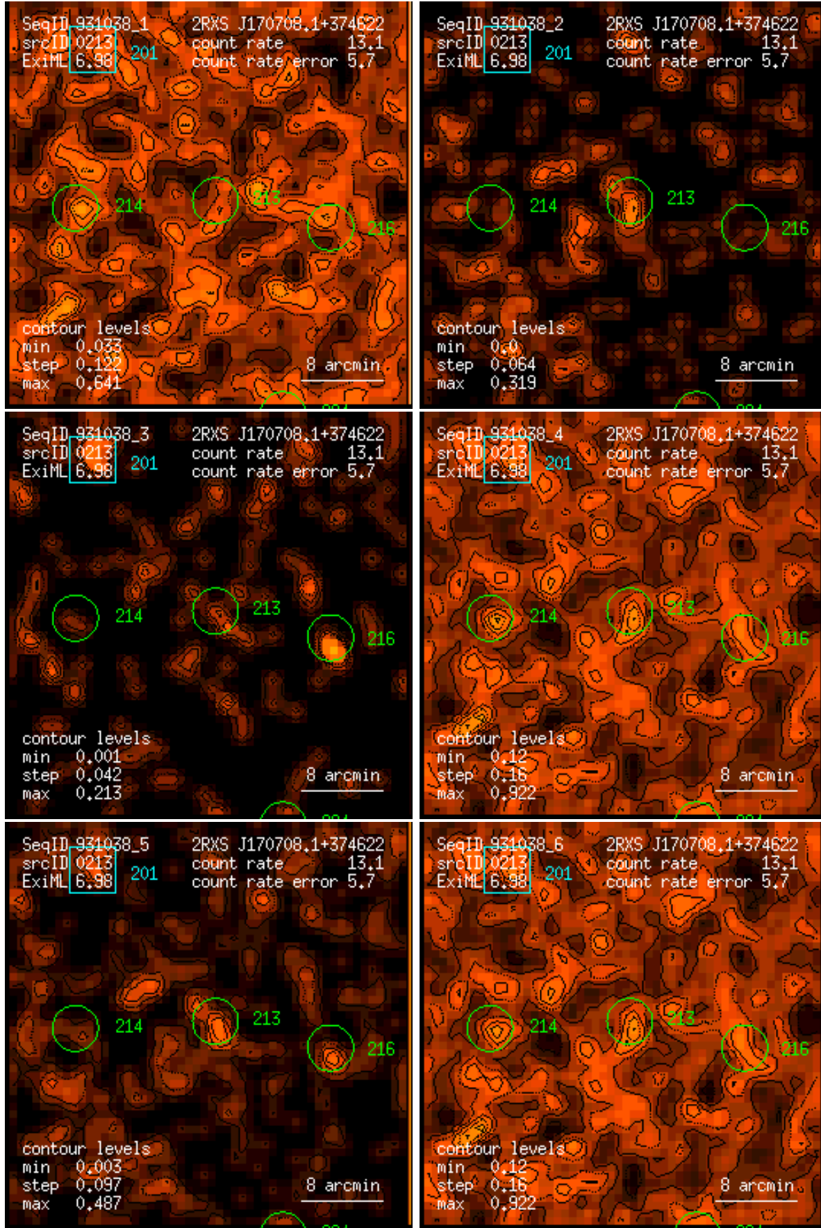
Figure 213: RASS 931038: detection 0213: band rate images, Gaussian filter: (1) PSPC channels 11 – 41, (2) 52 – 90, (3) 91 – 201, (4) 11 – 235, (5) 52 – 201, (6) 11 – 201. Broad band rates in counts/ks. Band rate contour levels in counts/ks/arcmin 2 .
