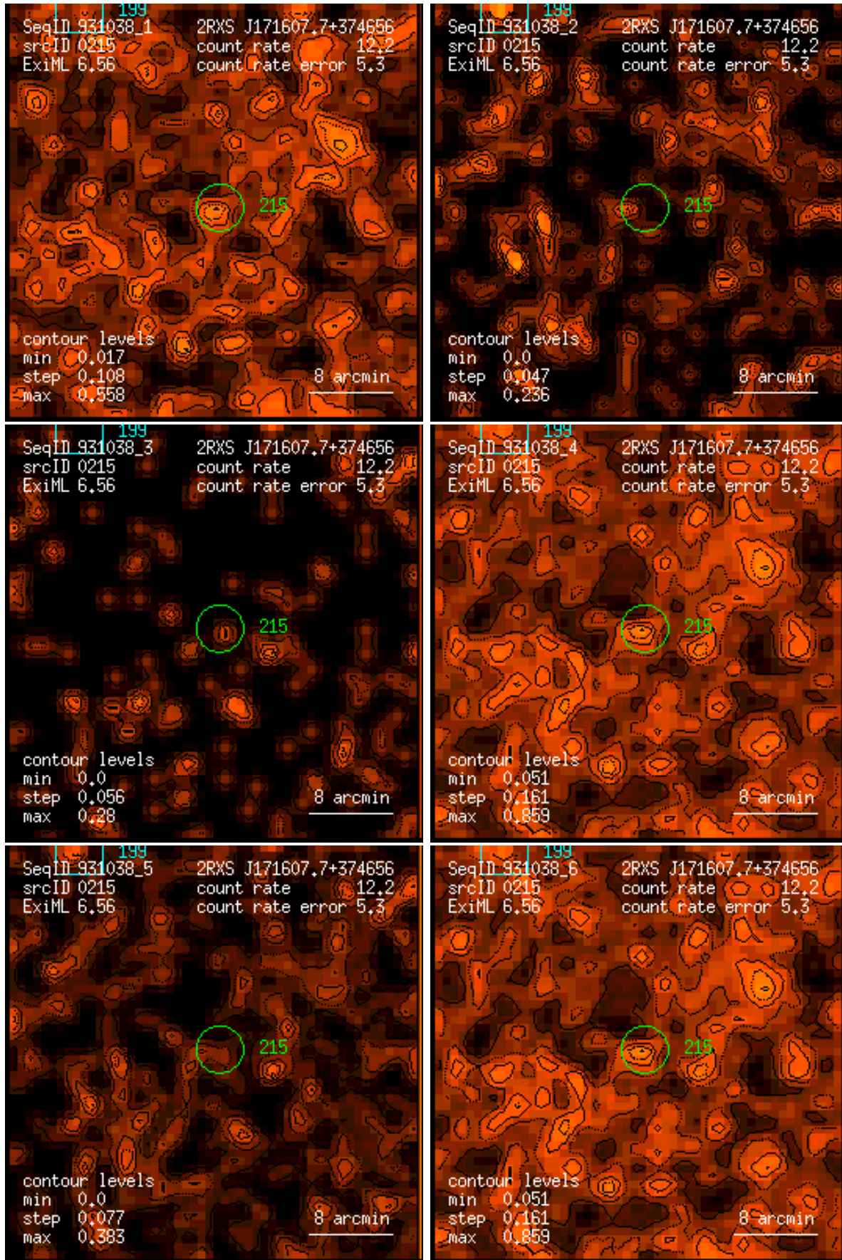
Figure 215: RASS 931038: detection 0215: band rate images, Gaussian filter: (1) PSPC channels 11 – 41, (2) 52 – 90, (3) 91 – 201, (4) 11 – 235, (5) 52 – 201, (6) 11 – 201. Broad band rates in counts/ks. Band rate contour levels in counts/ks/arcmin 2 .
