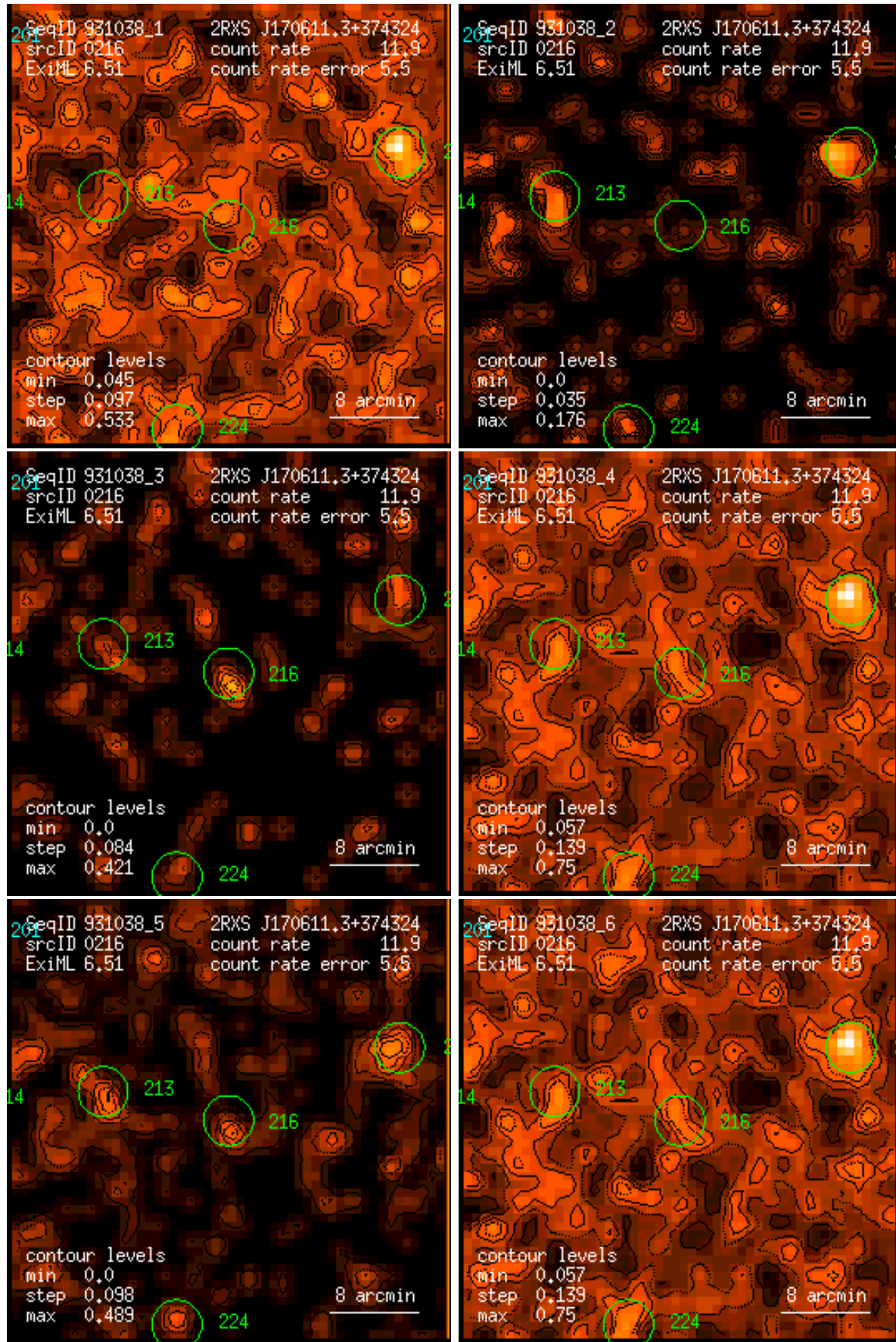
Figure 216: RASS 931038: detection 0216: band rate images, Gaussian filter: (1) PSPC channels 11 – 41, (2) 52 – 90, (3) 91 – 201, (4) 11 – 235, (5) 52 – 201, (6) 11 – 201. Broad band rates in counts/ks. Band rate contour levels in counts/ks/arcmin 2 .
