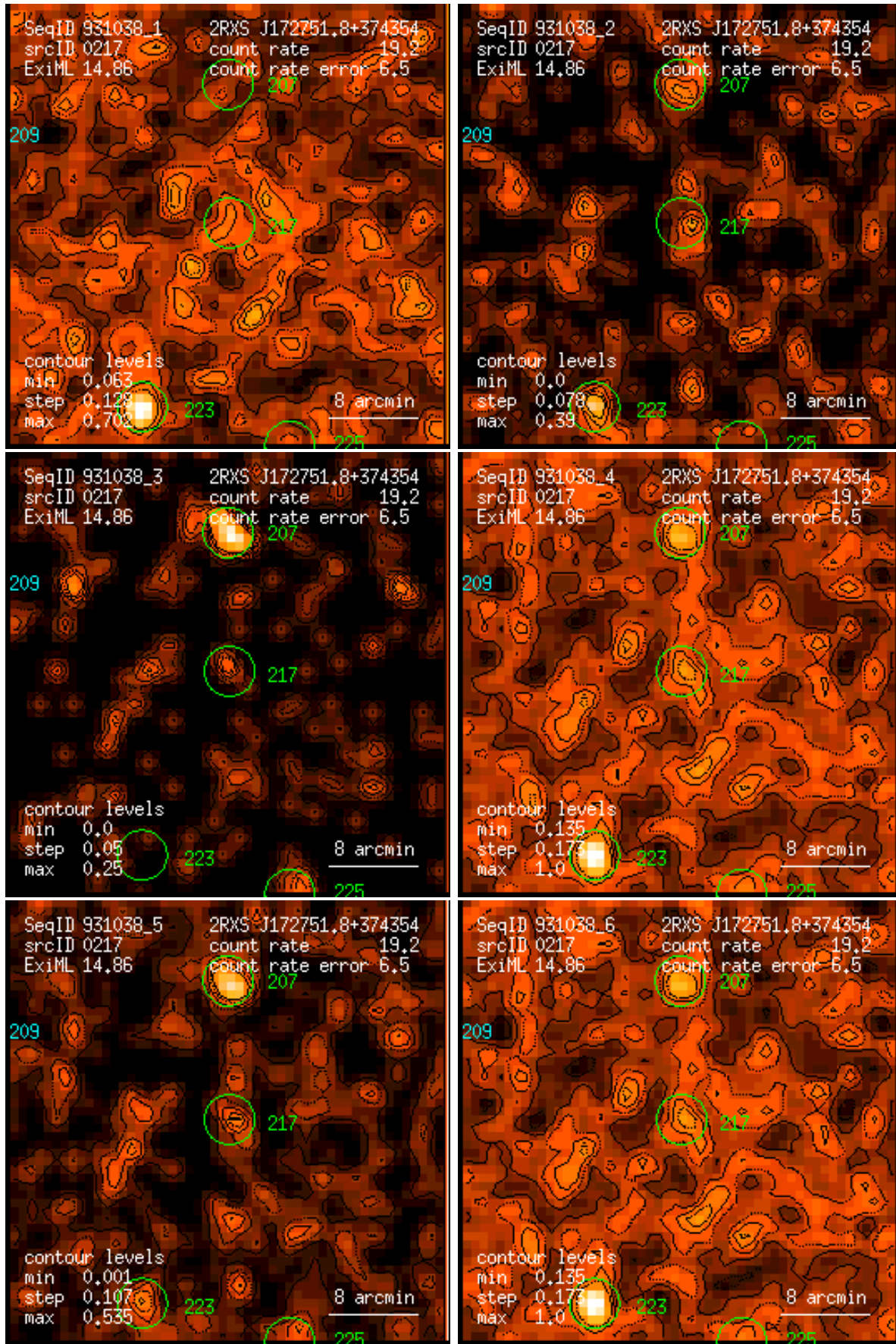
Figure 217: RASS 931038: detection 0217: band rate images, Gaussian filter: (1) PSPC channels 11 – 41, (2) 52 – 90, (3) 91 – 201, (4) 11 – 235, (5) 52 – 201, (6) 11 – 201. Broad band rates in counts/ks. Band rate contour levels in counts/ks/arcmin 2 .
