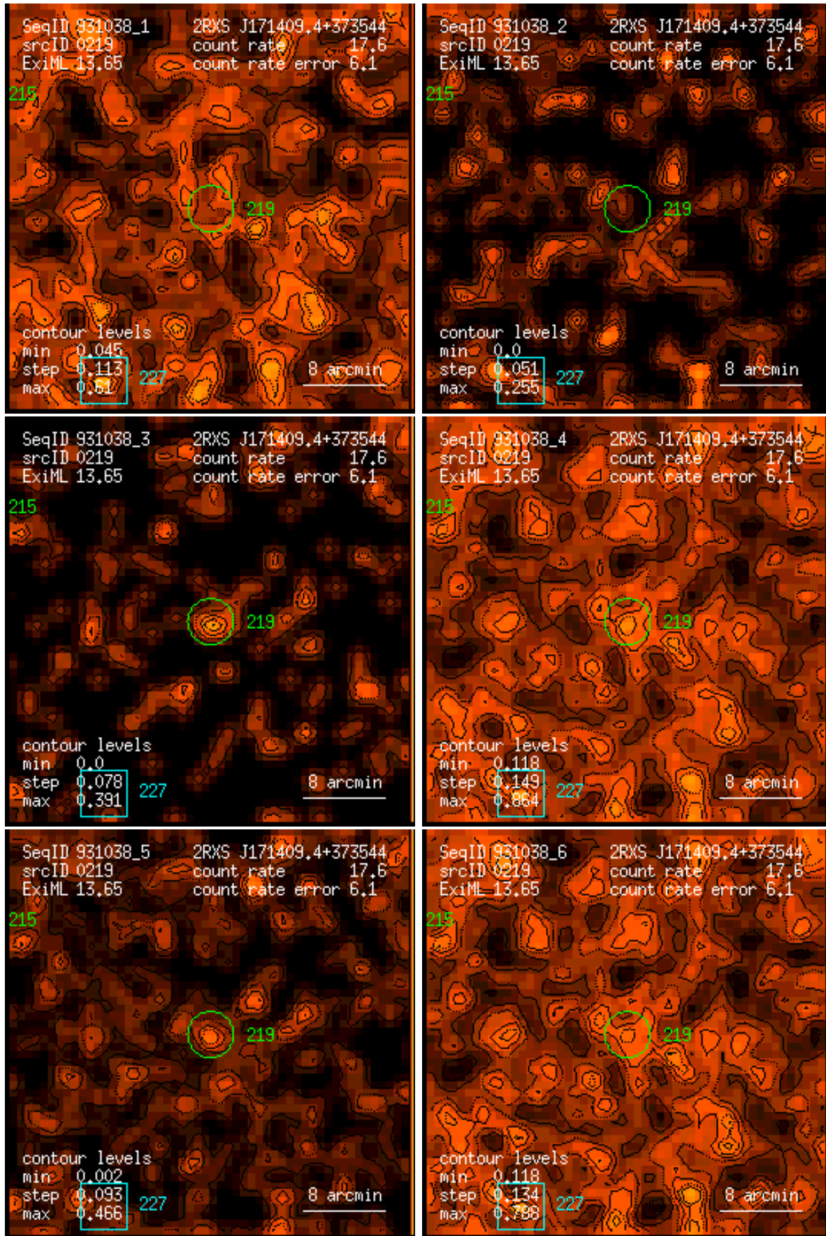
Figure 219: RASS 931038: detection 0219: band rate images, Gaussian filter: (1) PSPC channels 11 – 41, (2) 52 – 90, (3) 91 – 201, (4) 11 – 235, (5) 52 – 201, (6) 11 – 201. Broad band rates in counts/ks. Band rate contour levels in counts/ks/arcmin 2 .
