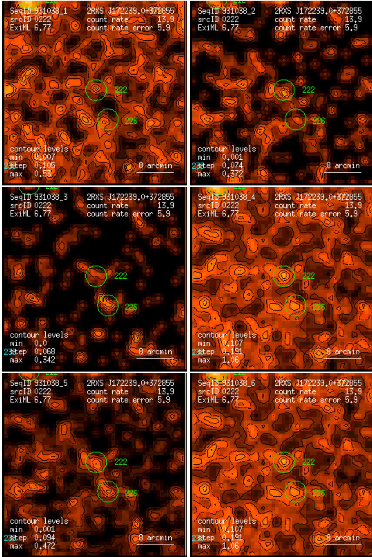
Figure 222: RASS 931038: detection 0222: band rate images, Gaussian filter: (1) PSPC channels 11 – 41, (2) 52 – 90, (3) 91 – 201, (4) 11 – 235, (5) 52 – 201, (6) 11 – 201. Broad band rates in counts/ks. Band rate contour levels in counts/ks/arcmin 2 .
