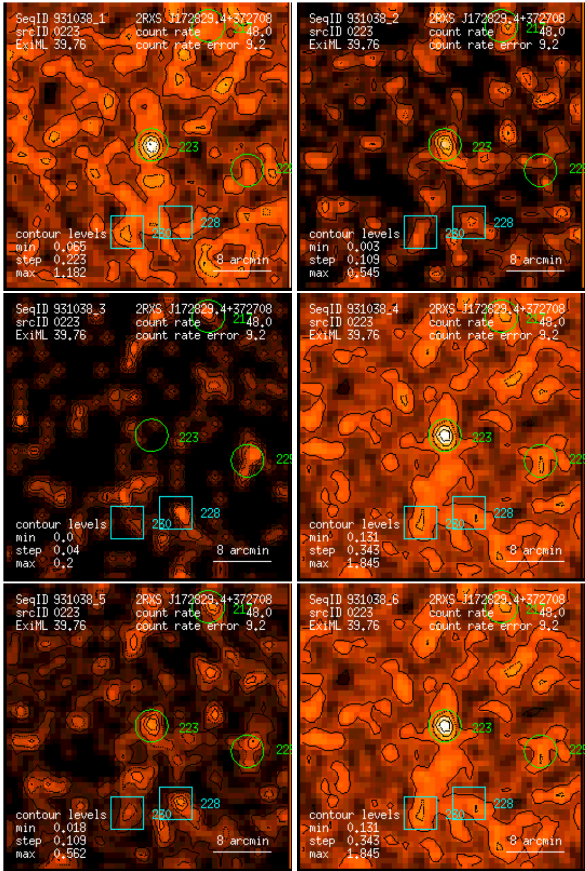
Figure 223: RASS 931038: detection 0223: band rate images, Gaussian filter: (1) PSPC channels 11 – 41, (2) 52 – 90, (3) 91 – 201, (4) 11 – 235, (5) 52 – 201, (6) 11 – 201. Broad band rates in counts/ks. Band rate contour levels in counts/ks/arcmin 2 .
