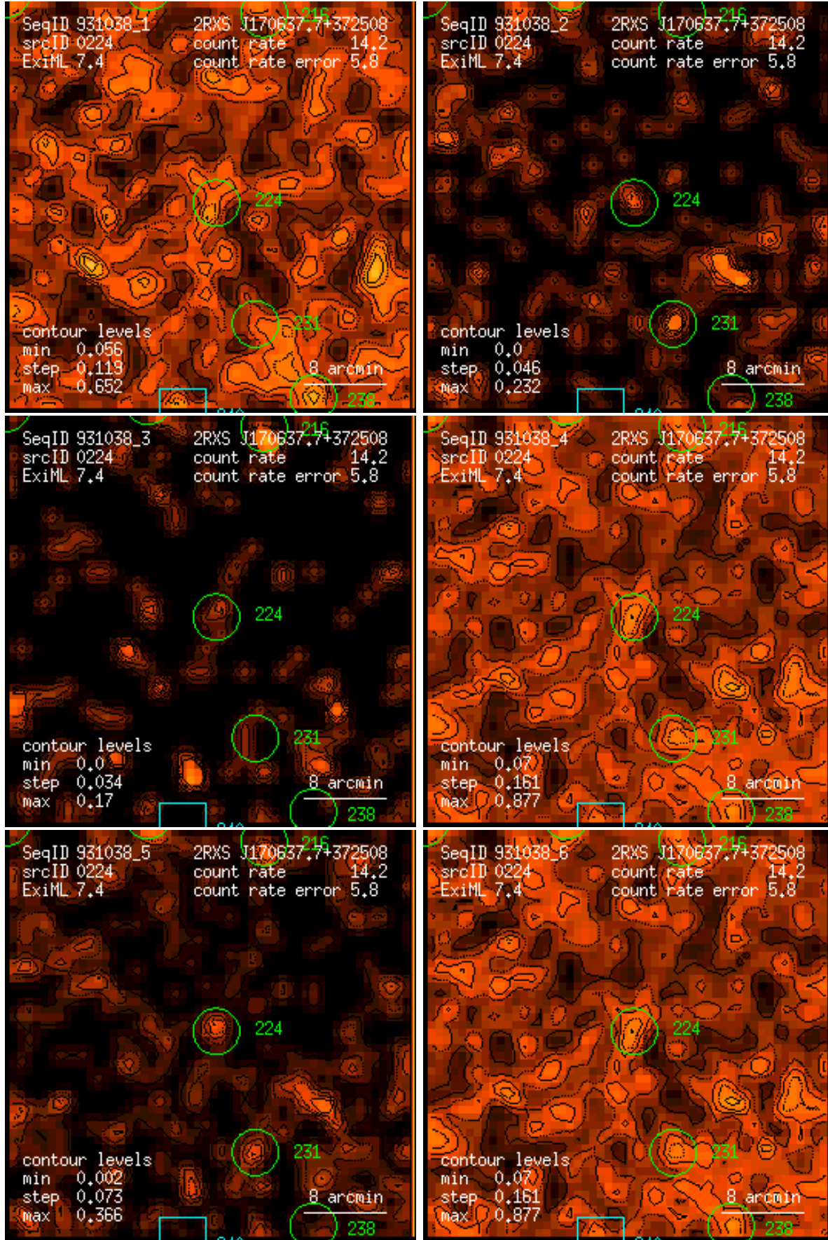
Figure 224: RASS 931038: detection 0224: band rate images, Gaussian filter: (1) PSPC channels 11 – 41, (2) 52 – 90, (3) 91 – 201, (4) 11 – 235, (5) 52 – 201, (6) 11 – 201. Broad band rates in counts/ks. Band rate contour levels in counts/ks/arcmin 2 .
