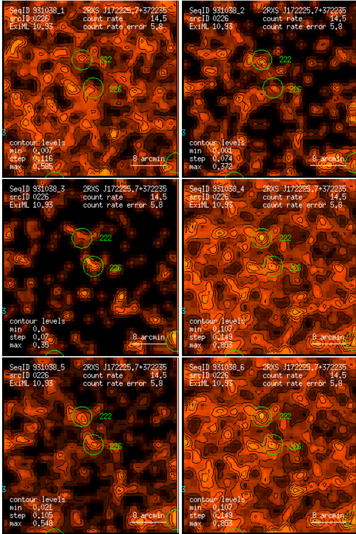
Figure 226: RASS 931038: detection 0226: band rate images, Gaussian filter: (1) PSPC channels 11 – 41, (2) 52 – 90, (3) 91 – 201, (4) 11 – 235, (5) 52 – 201, (6) 11 – 201. Broad band rates in counts/ks. Band rate contour levels in counts/ks/arcmin 2 .
